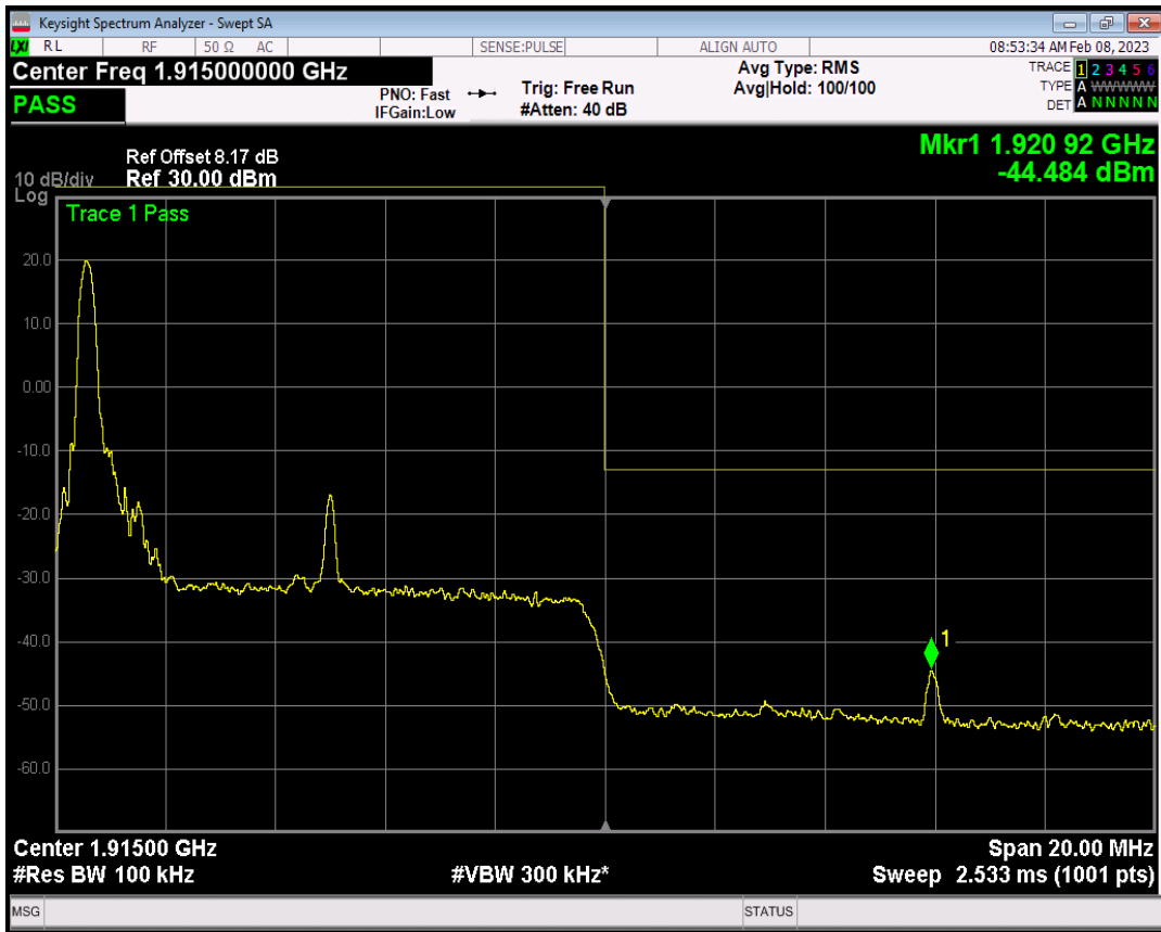
Band25 QAM16 BW=10MHz Channel=26640 RB Size=1 Position=#Max
