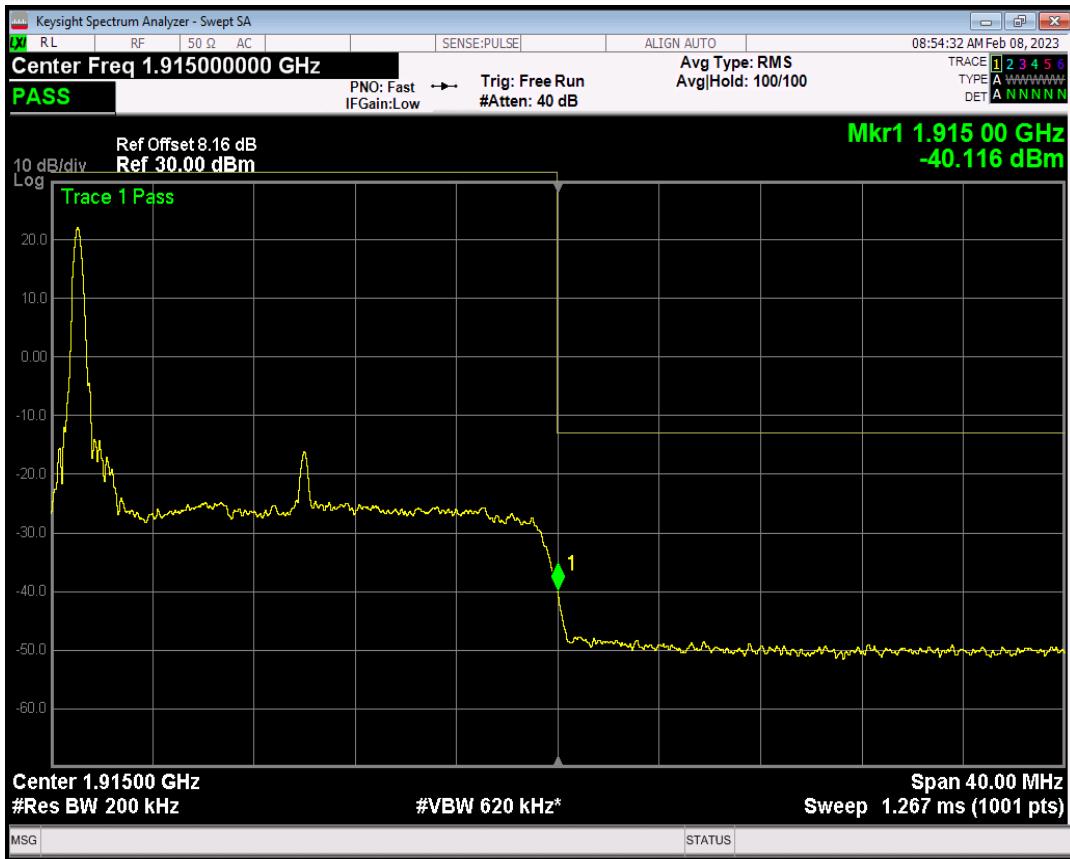
Band25 QAM16 BW=20MHz Channel=26590 RB Size=1 Position=#Max
