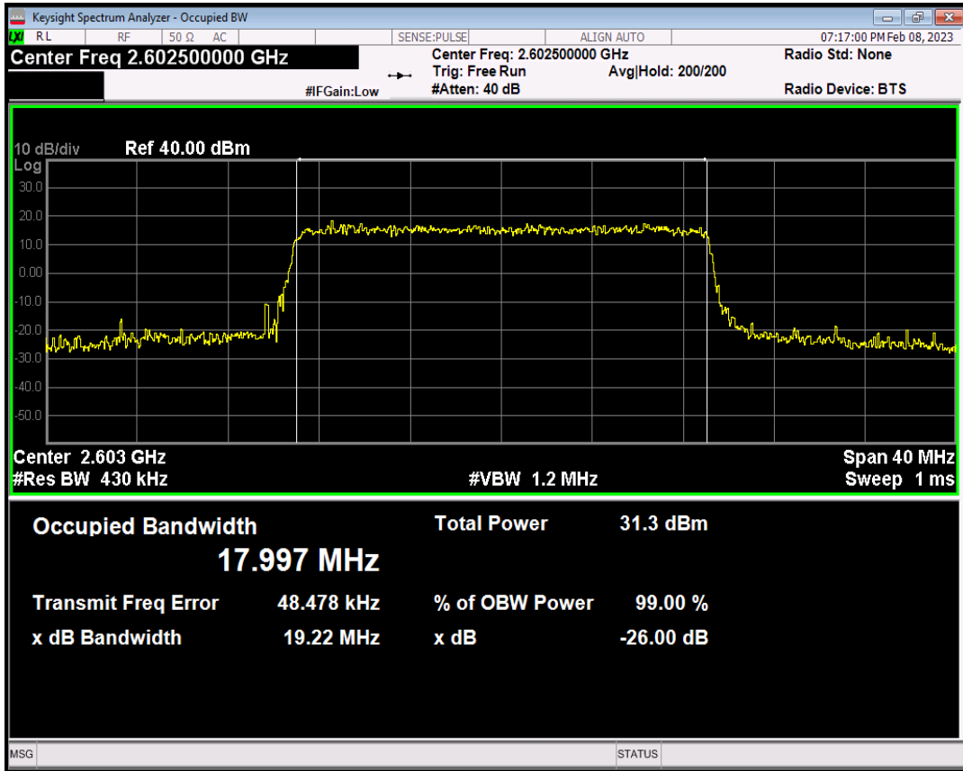
Band41 QAM16 BW=20MHz Channel=40715 RB Size=100 Position=#0
