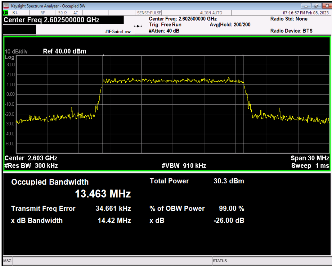
Band41 QAM16 BW=15MHz Channel=40715 RB Size=75 Position=#0
