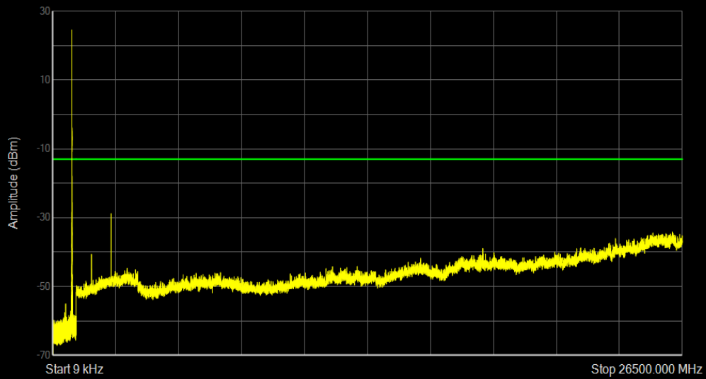
Band26(824-849) QPSK BW=3MHz Channel=26805 RB Size=1 Position=#0
