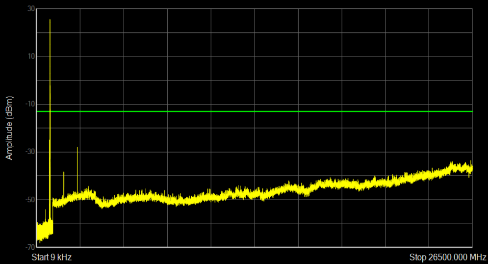
Band26(824-849) QPSK BW=15MHz Channel=26965 RB Size=1 Position=#0
