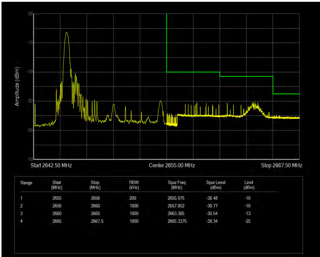
Band41(2555-2655) 16QAM BW=10MHz Channel=41190 RB Size=1 Position=#Max
