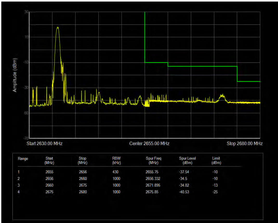
Band41(2555-2655) 16QAM BW=20MHz Channel=41140 RB Size=1 Position=#Max
