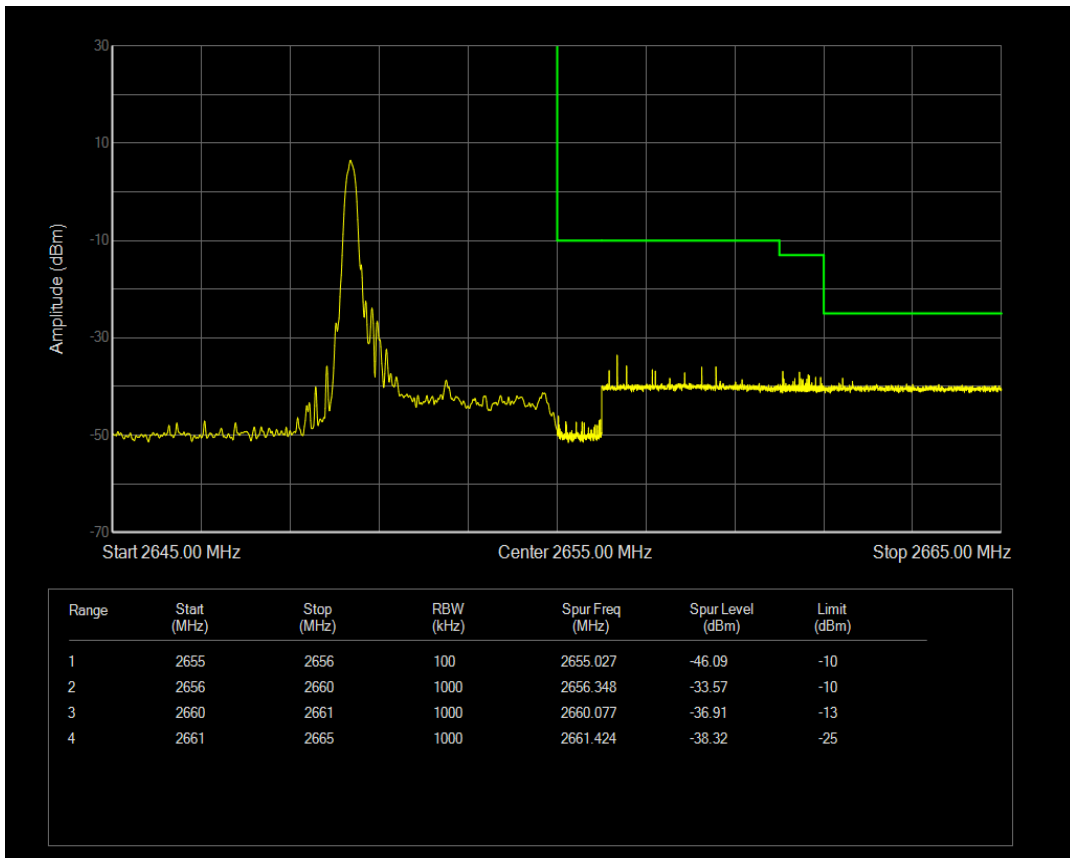
Band41(2555-2655) QAM16 BW=5MHz Channel=41215 RB Size=1 Position=#Max
