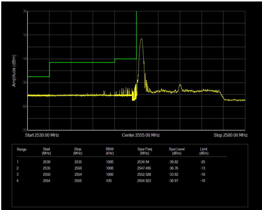
Band41(2555-2655) QAM16 BW=20MHz Channel=40340 RB Size=1 Position=#Max
