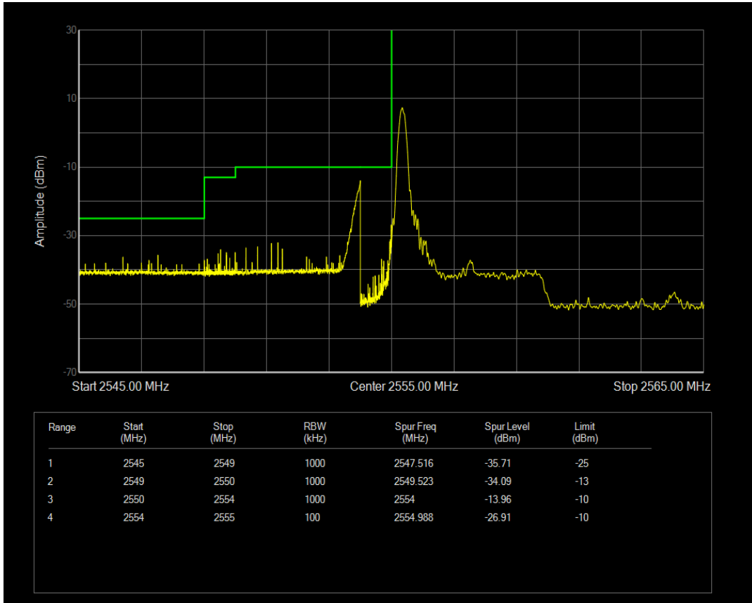
Band41(2555-2655) QPSK BW=5MHz Channel=40265 RB Size=1 Position=#Max
