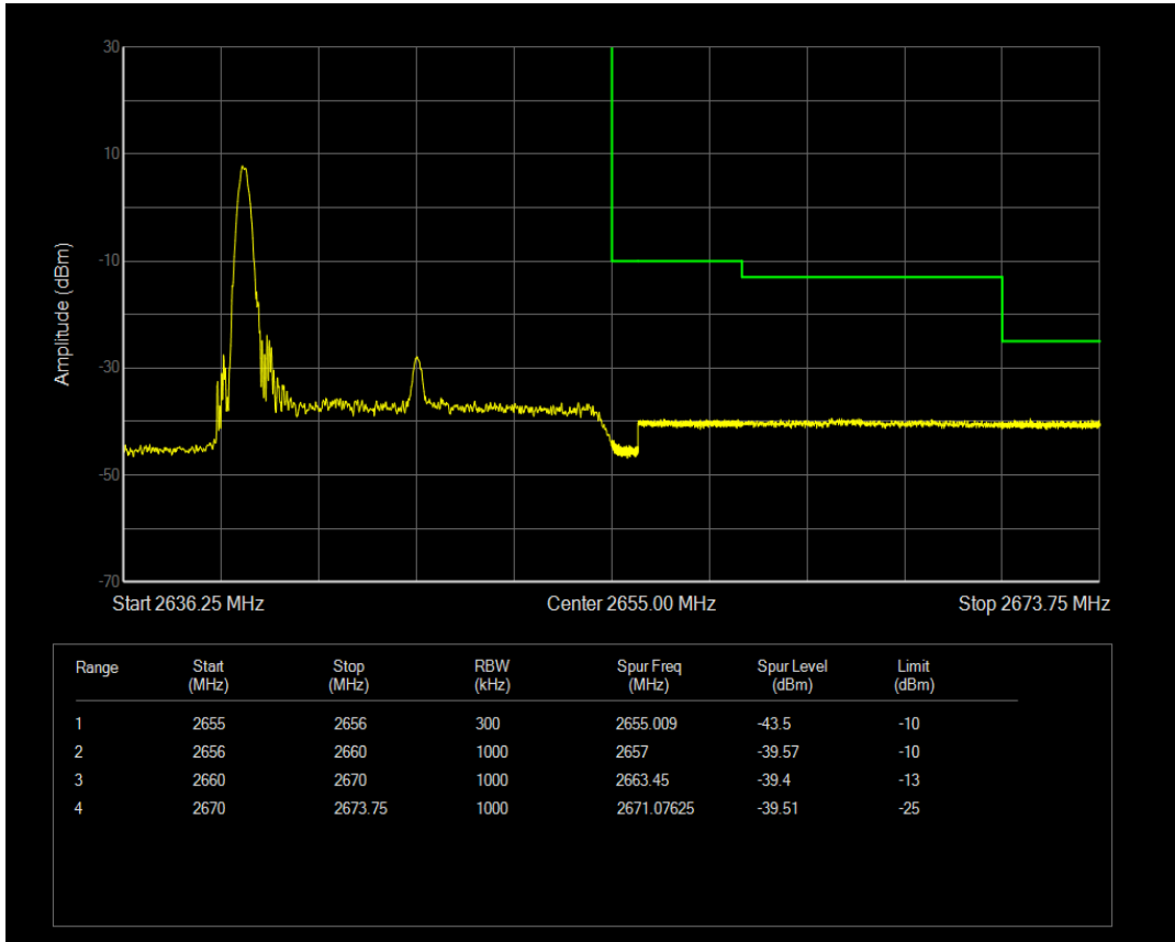
Band41(2555-2655) QPSK BW=15MHz Channel=41165 RB Size=1 Position=#Max
