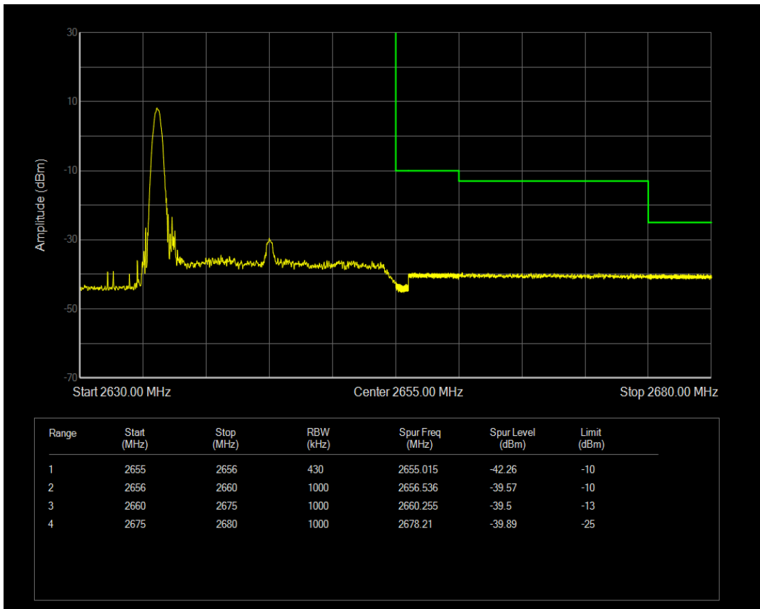
Band41(2555-2655) QAM16 BW=20MHz Channel=41140 RB Size=1 Position=#Max
