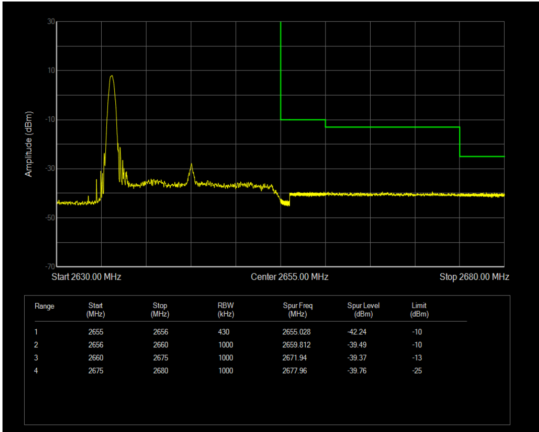
Band41(2555-2655) QPSK BW=20MHz Channel=41140 RB Size=1 Position=#Max
