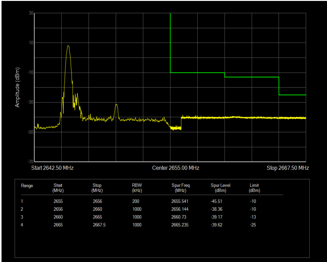
Band41(2555-2655) QPSK BW=10MHz Channel=41190 RB Size=1 Position=#Max
