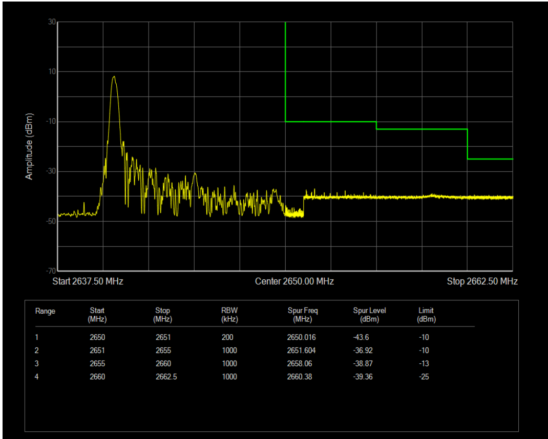
Band41(2540-2650) QAM16 BW=10MHz Channel=41140 RB Size=1 Position=#Max
