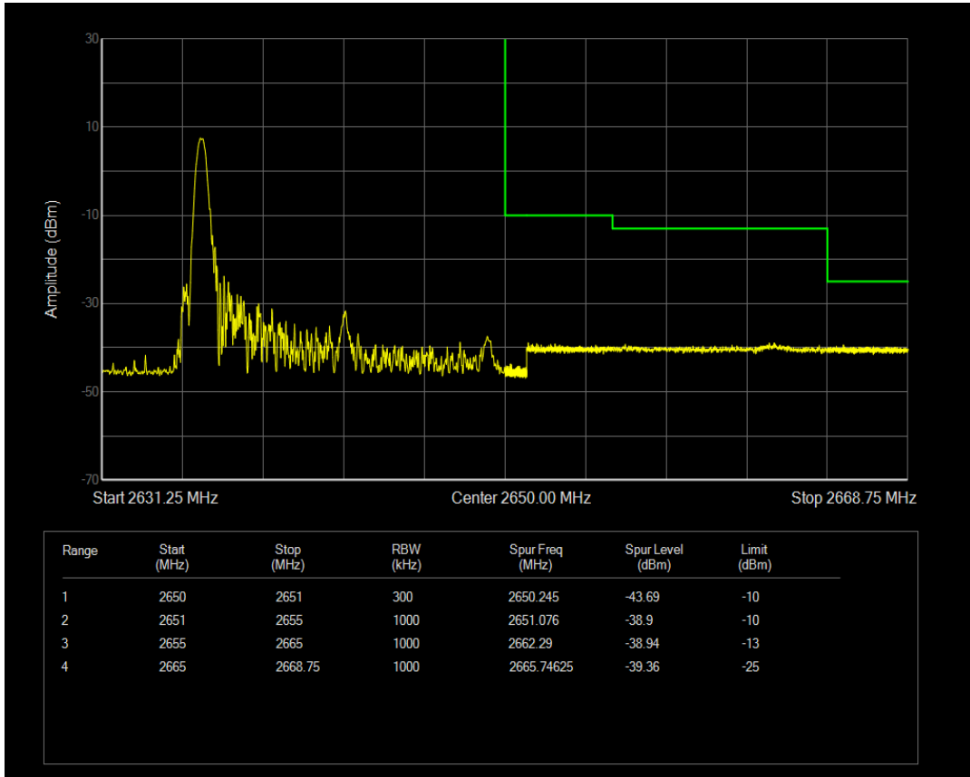
Band41(2540-2650) QAM16 BW=15MHz Channel=41115 RB Size=1 Position=#Max
