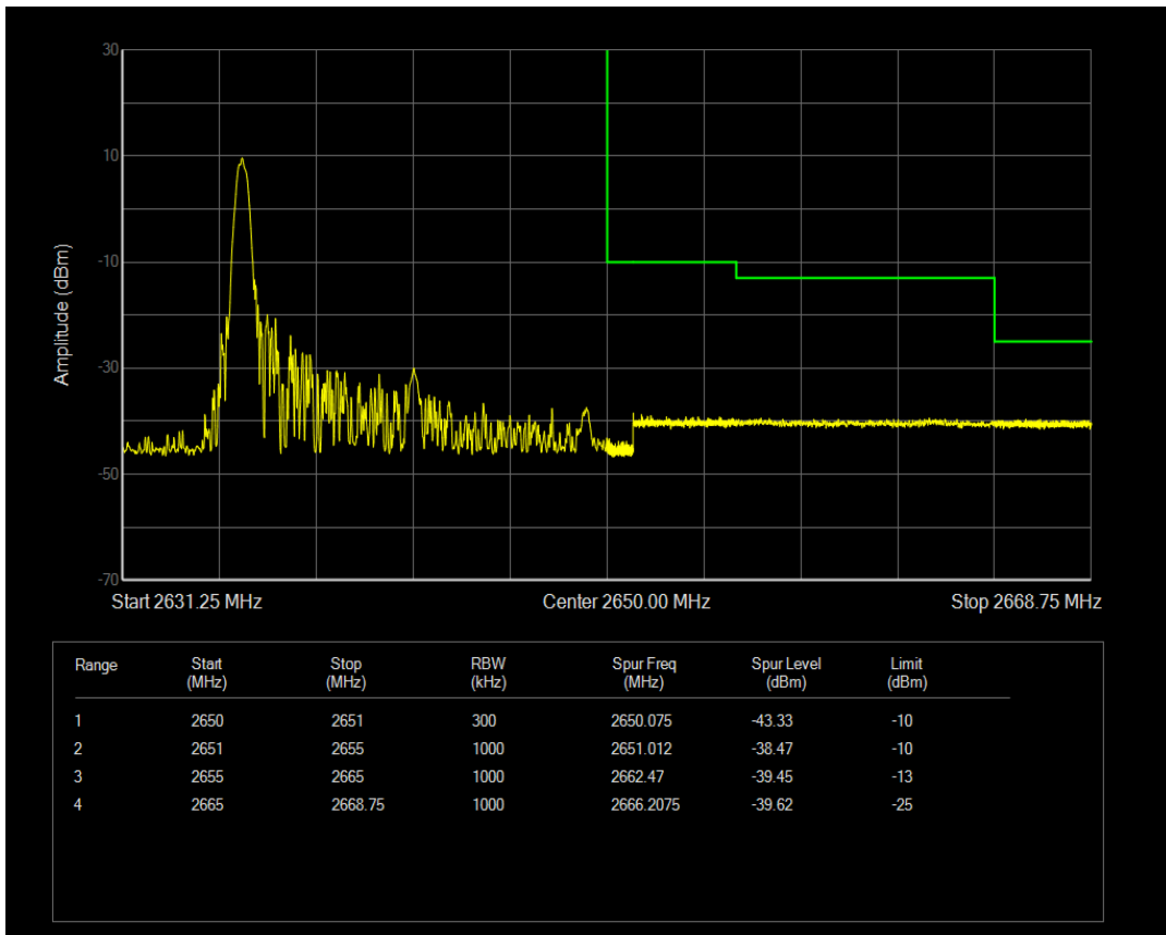
Band41(2540-2650) QPSK BW=15MHz Channel=41115 RB Size=1 Position=#Max
