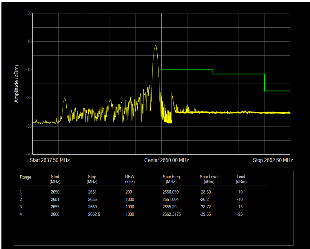
Band41(2540-2650) QAM16 BW=10MHz Channel=41140 RB Size=50 Position=#0
