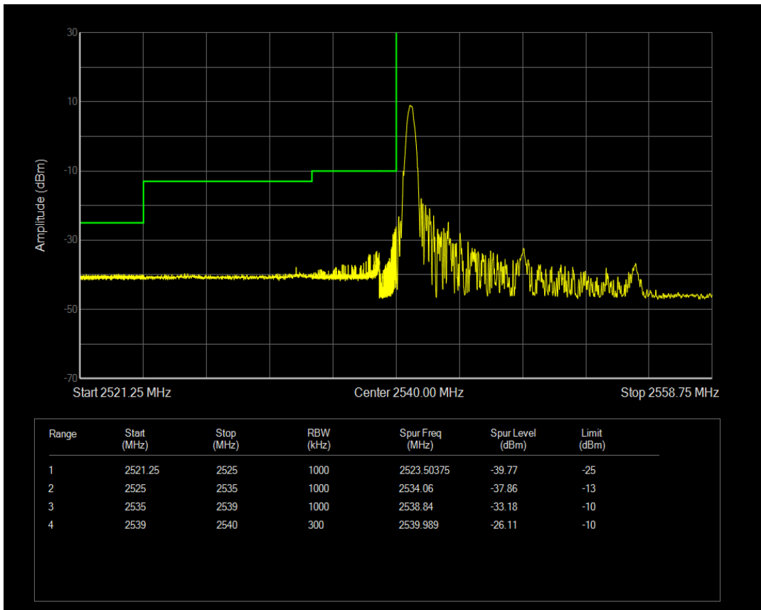
Band41(2540-2650) QPSK BW=15MHz Channel=40165 RB Size=1 Position=#Max
