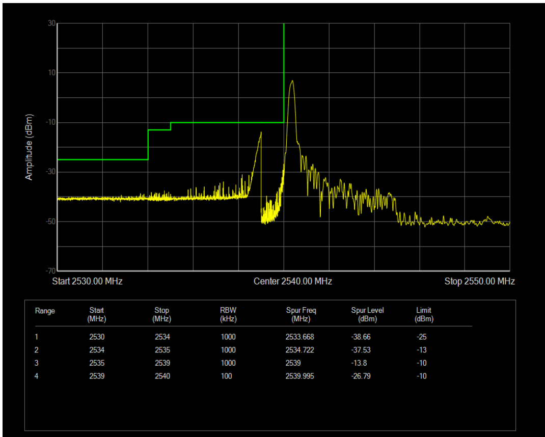
Band41(2540-2650) QPSK BW=5MHz Channel=40115 RB Size=1 Position=#Max
