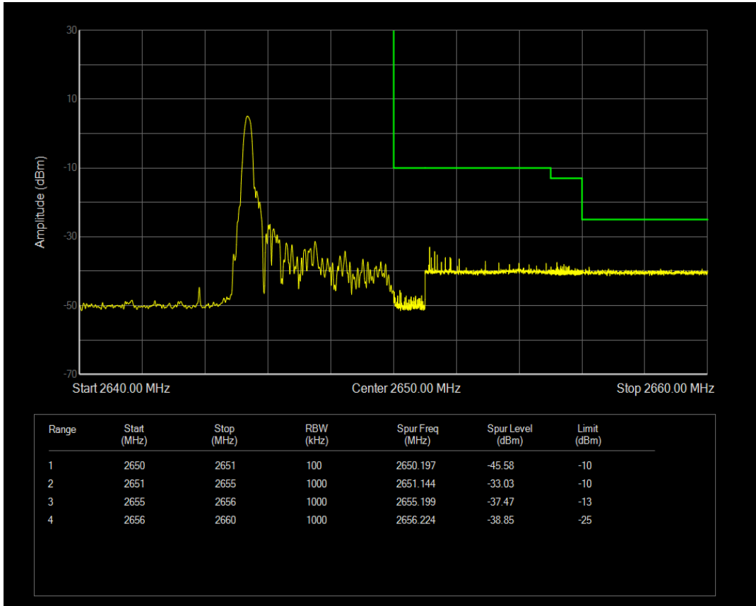
Band41(2540-2650) QAM16 BW=5MHz Channel=41165 RB Size=1 Position=#Max
