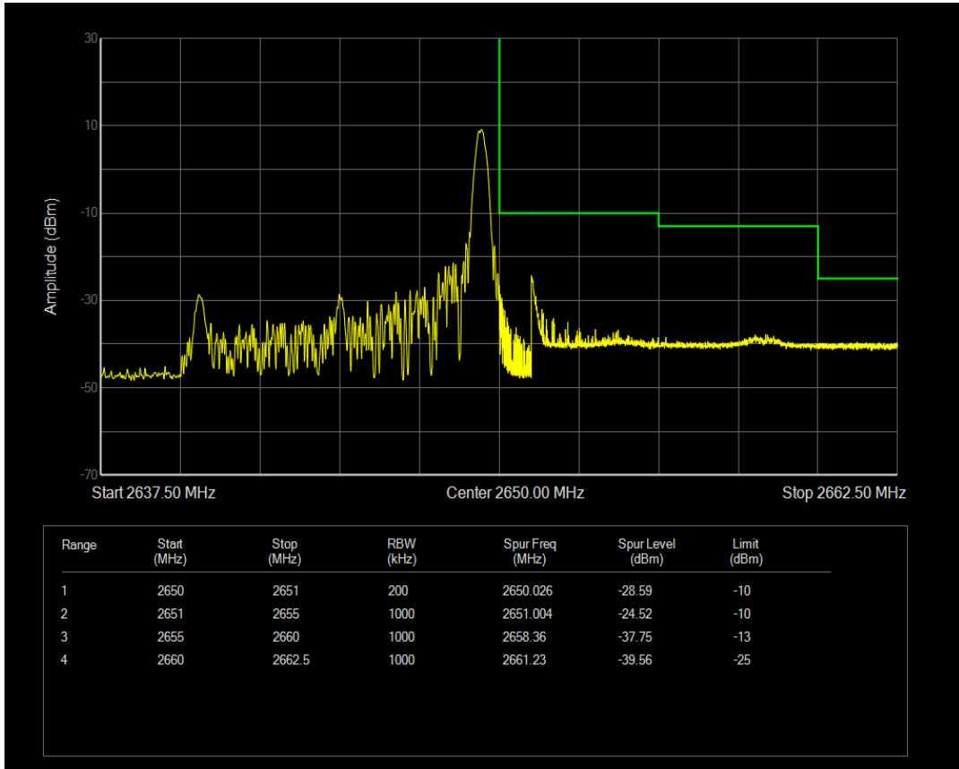
Band41(2540-2650) QPSK BW=10MHz Channel=41140 RB Size=50 Position=#0
