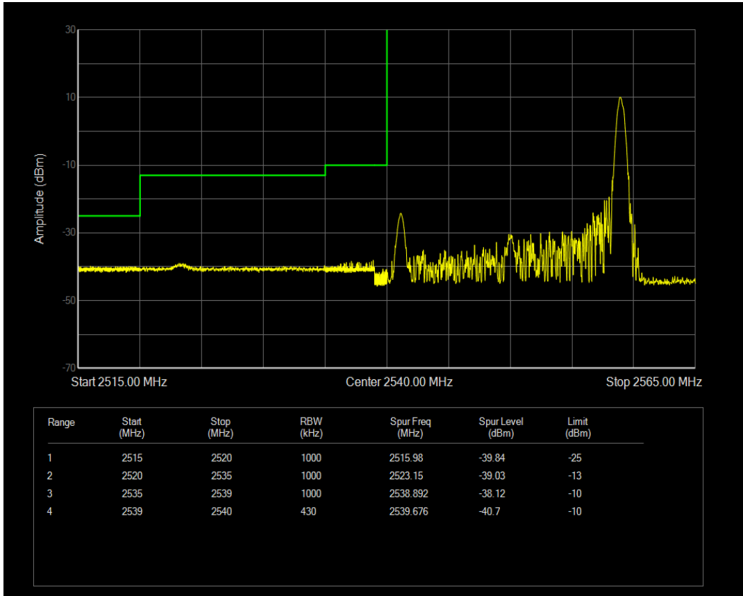
Band41(2540-2650) QPSK BW=20MHz Channel=40190 RB Size=100 Position=#0
