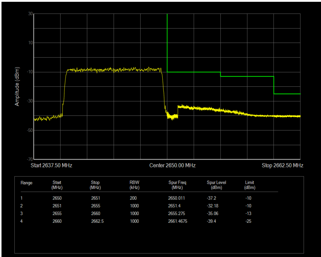
Band41(2540-2650) QAM16 BW=10MHz Channel=41140 RB Size=1 Position=#0
