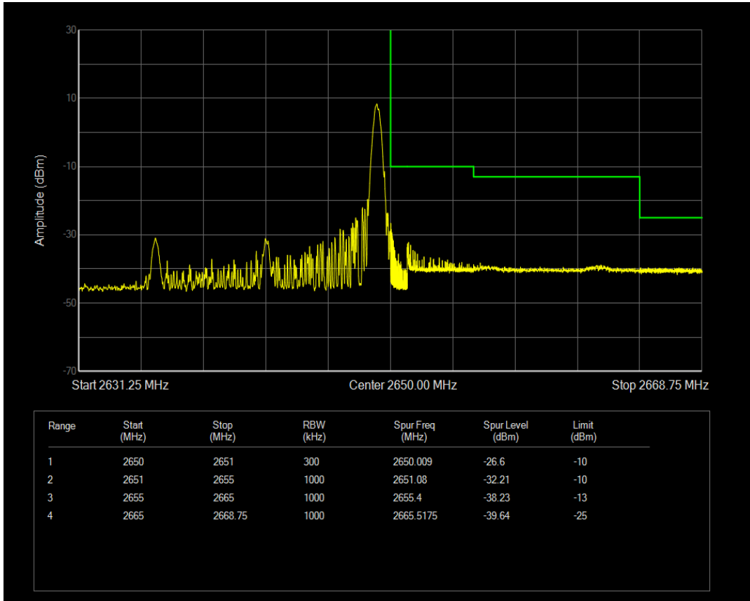
Band41(2540-2650) QPSK BW=15MHz Channel=41115 RB Size=75 Position=#0
