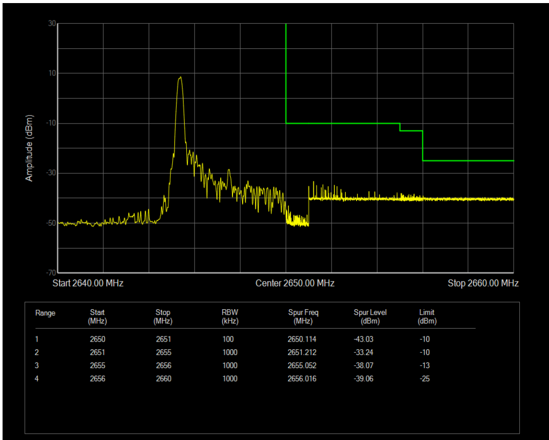
Band41(2540-2650) QPSK BW=5MHz Channel=41165 RB Size=1 Position=#Max
