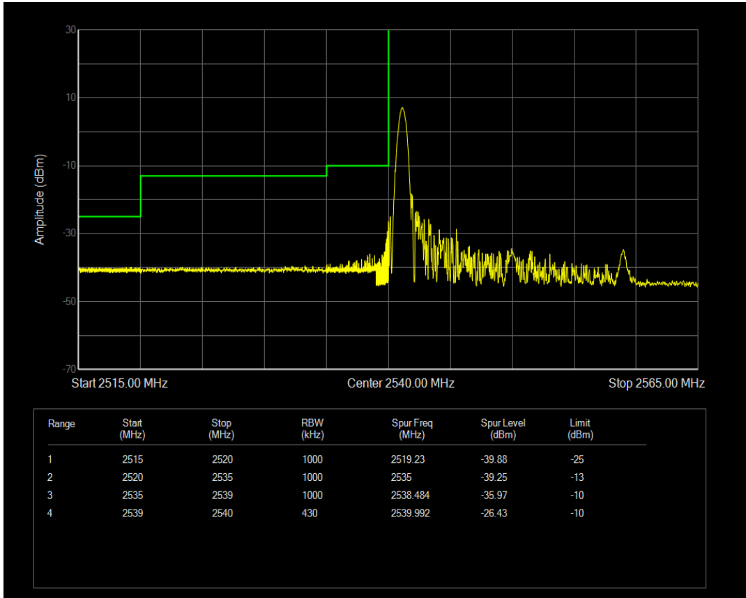
Band41(2540-2650) QAM16 BW=20MHz Channel=40190 RB Size=1 Position=#Max
