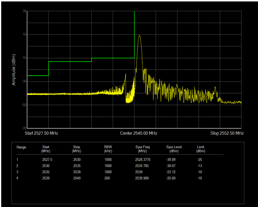
Band41(2540-2650) QPSK BW=10MHz Channel=40140 RB Size=1 Position=#Max
