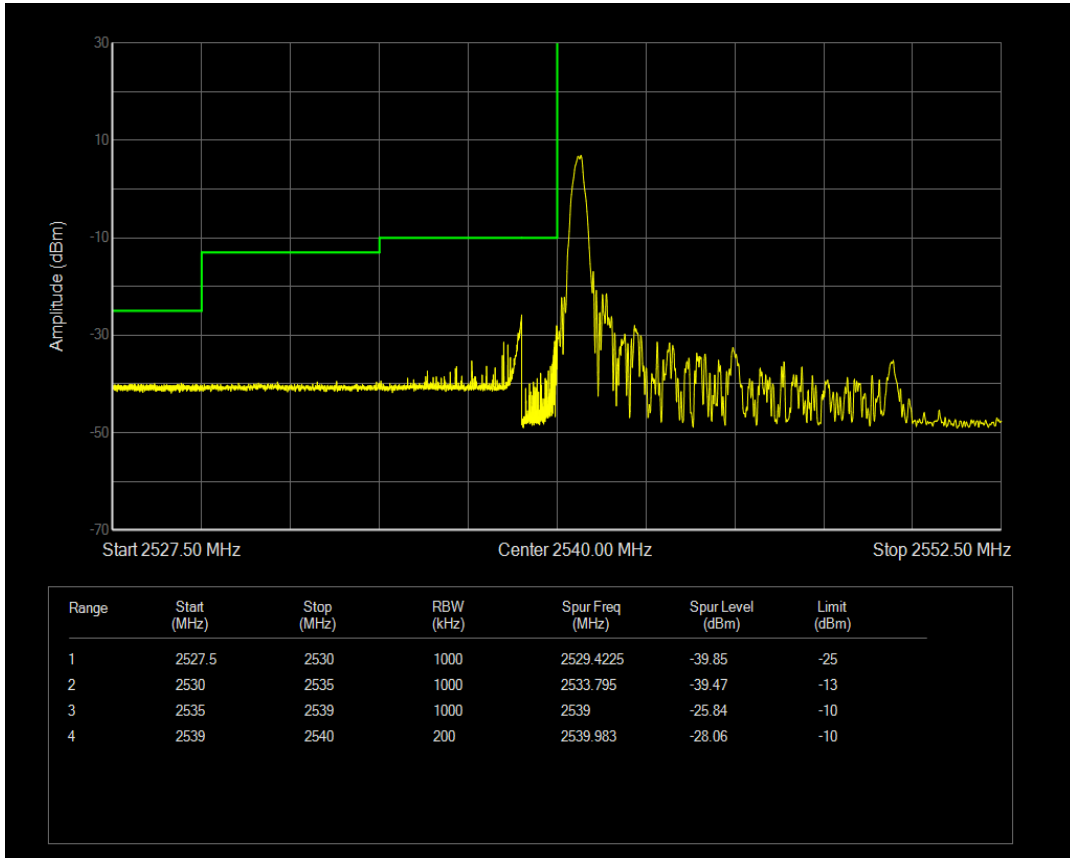
Band41(2540-2650) QAM16 BW=10MHz Channel=40140 RB Size=1 Position=#Max
