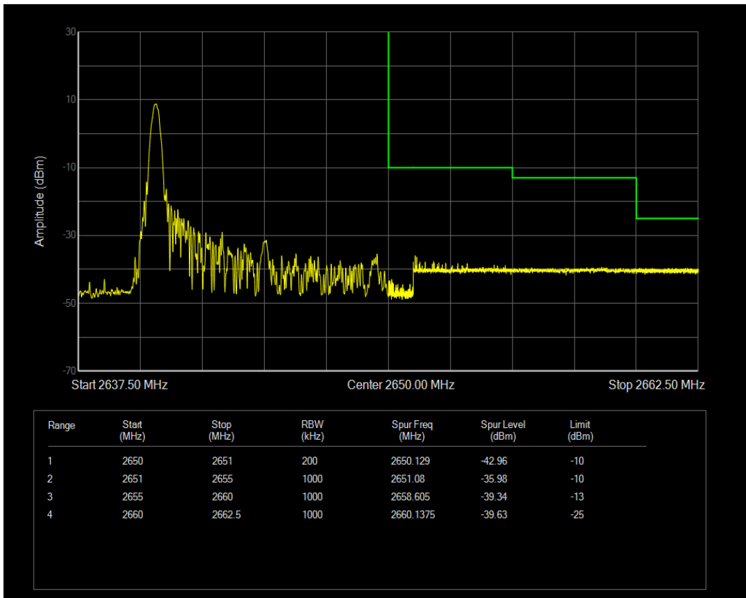
Band41(2540-2650) QPSK BW=10MHz Channel=41140 RB Size=1 Position=#Max
