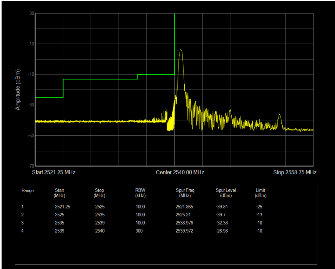
Band41(2540-2650) QAM16 BW=15MHz Channel=40165 RB Size=1 Position=#Max
