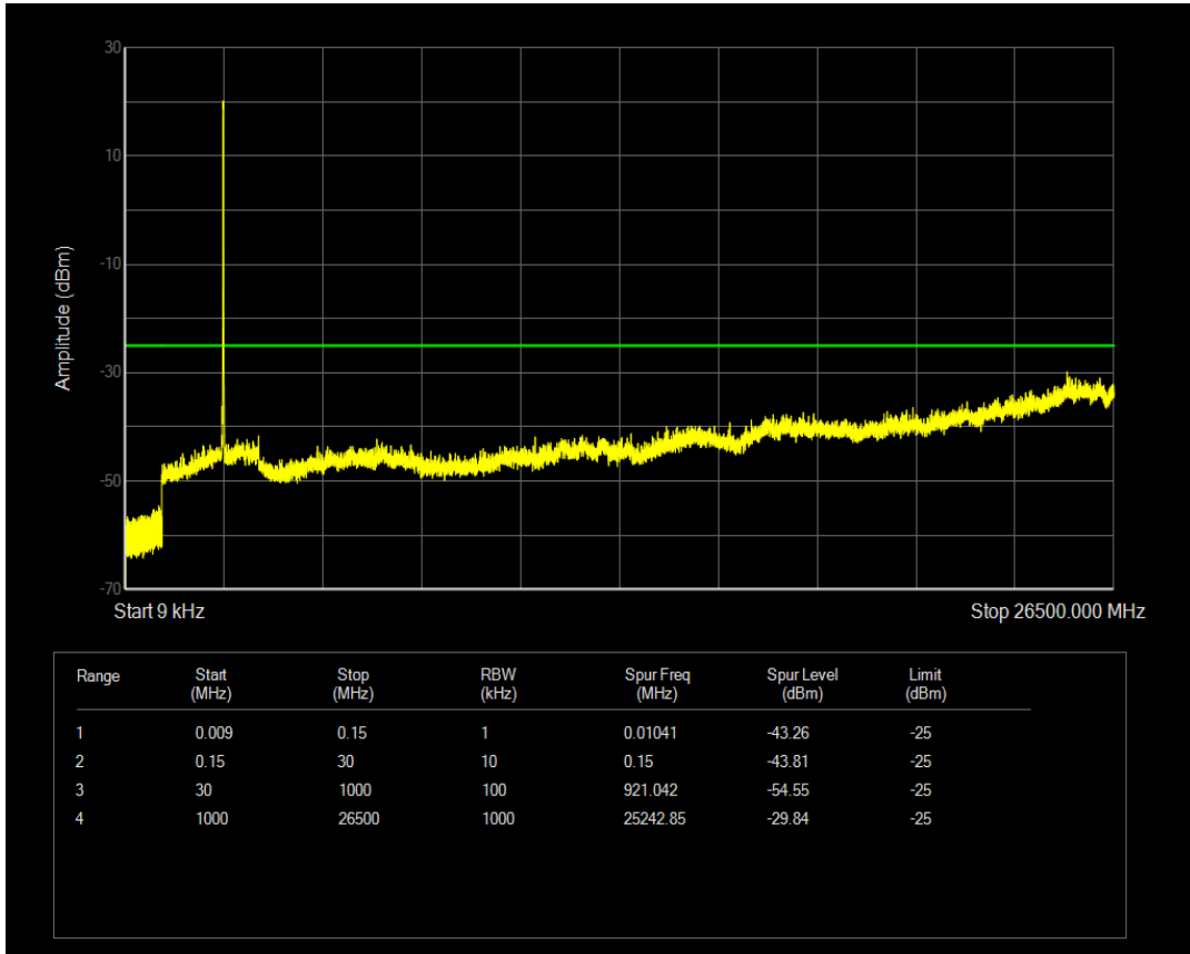
Band41(2540-2650) QPSK BW=15MHz Channel=40165 RB Size=1 Position=#0
