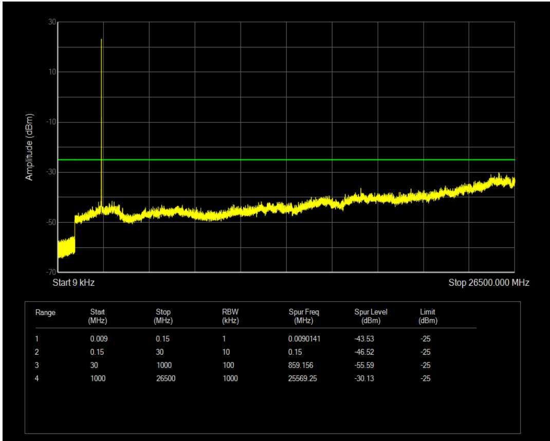
Band41(2540-2650) QAM16 BW=5MHz Channel=40115 RB Size=1 Position=#0
