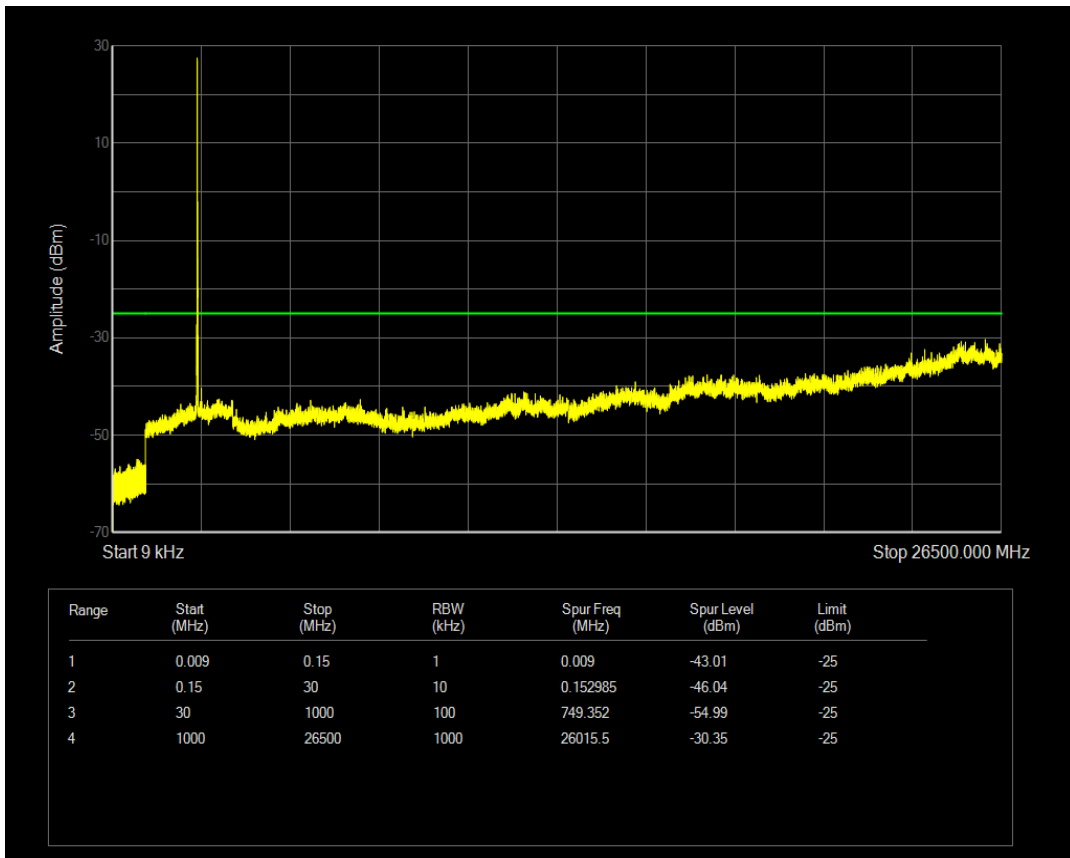
Band41(2540-2650) QPSK BW=15MHz Channel=40165 RB Size=75 Position=#0
