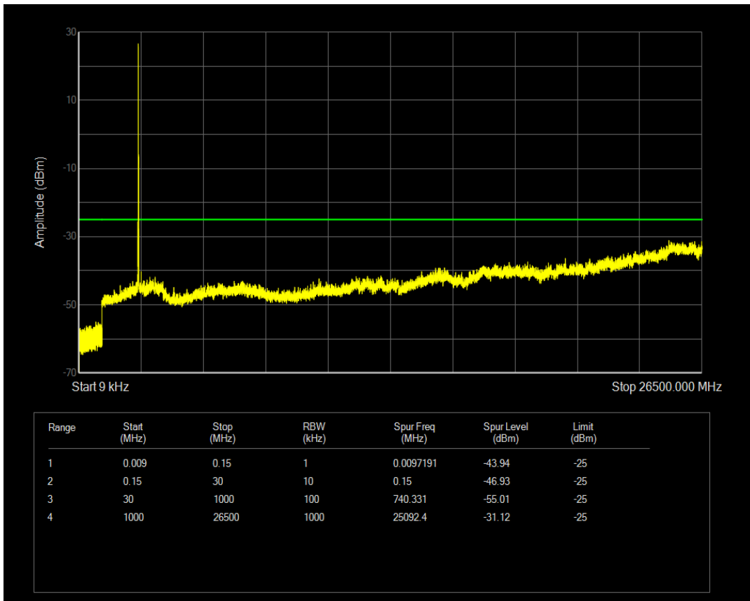
Band41(2540-2650) QAM16 BW=15MHz Channel=40165 RB Size=75 Position=#0
