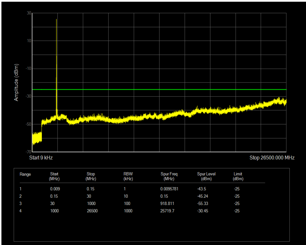
Band41(2540-2650) QAM16 BW=20MHz Channel=40190 RB Size=100 Position=#0
