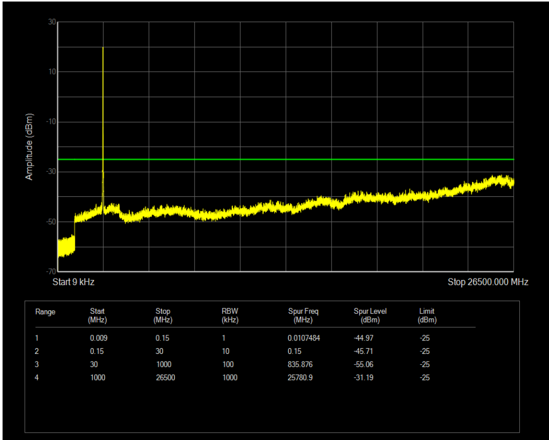
Band41(2540-2650) QAM16 BW=15MHz Channel=41115 RB Size=1 Position=#0
