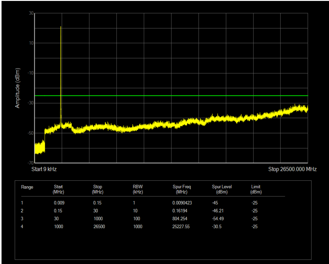
Band41(2540-2650) QAM16 BW=15MHz Channel=40165 RB Size=1 Position=#0
