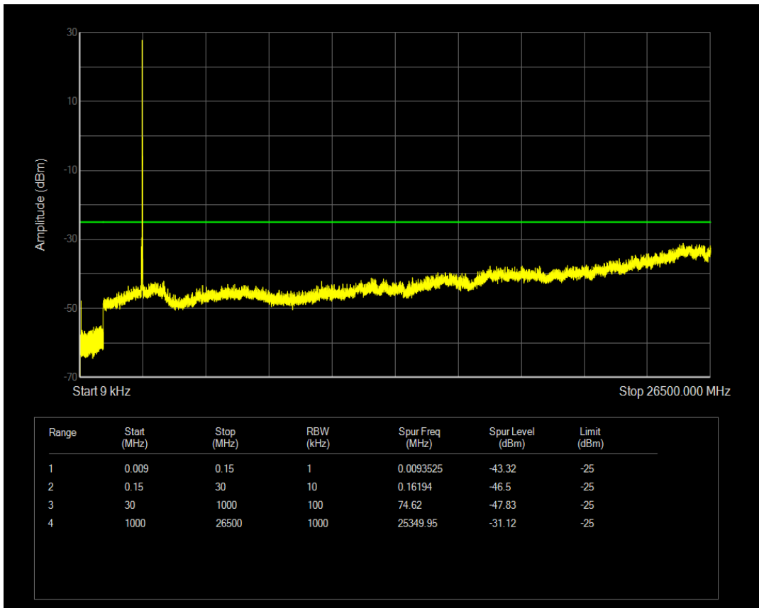
Band41(2540-2650) QAM16 BW=15MHz Channel=41115 RB Size=75 Position=#0
