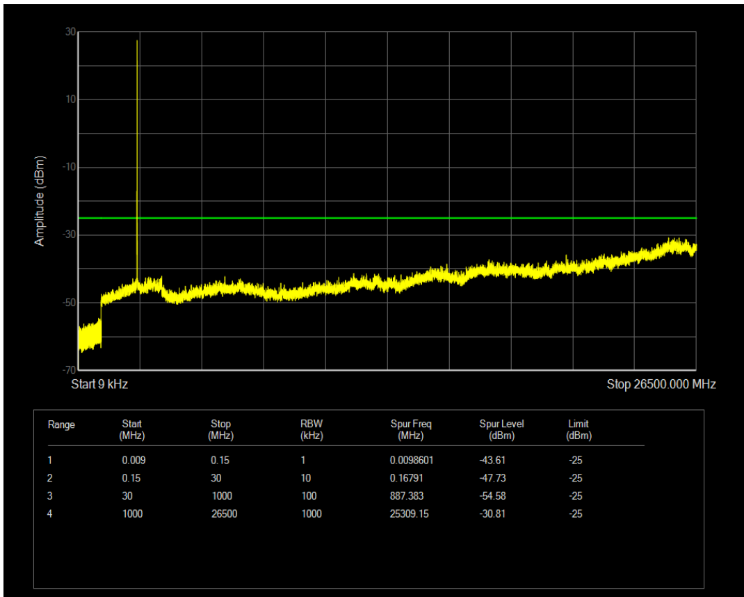
Band41(2540-2650) QPSK BW=5MHz Channel=40115 RB Size=25 Position=#0
