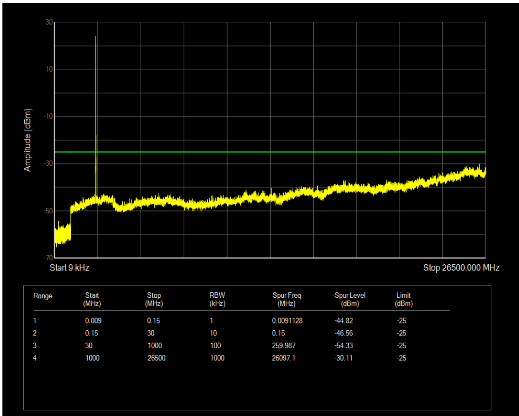
Band41(2540-2650) QAM16 BW=10MHz Channel=40140 RB Size=50 Position=#0
