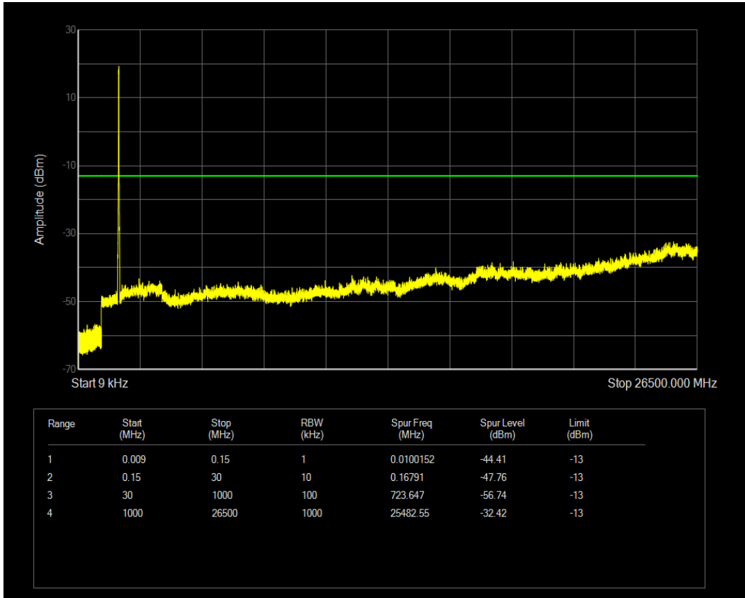
Band41(2540-2650) QPSK BW=5MHz Channel=40115 RB Size=1 Position=#0
