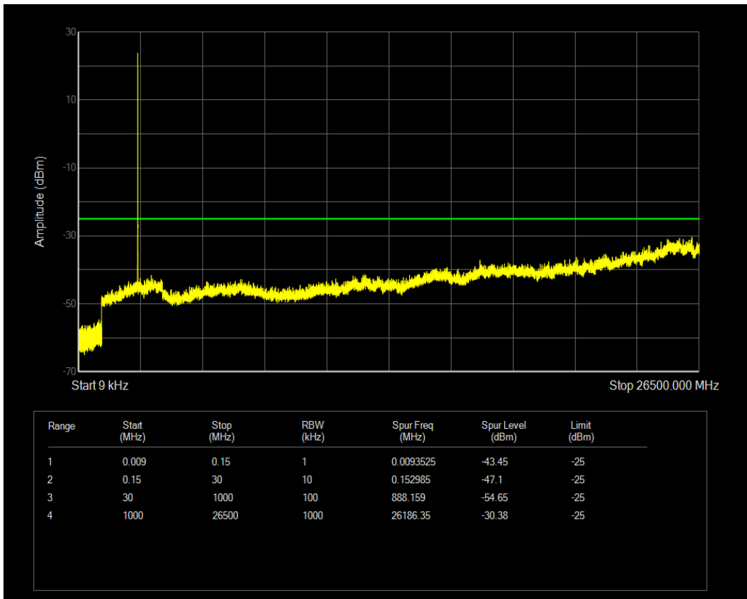
Band41(2540-2650) QAM16 BW=5MHz Channel=40115 RB Size=25 Position=#0
