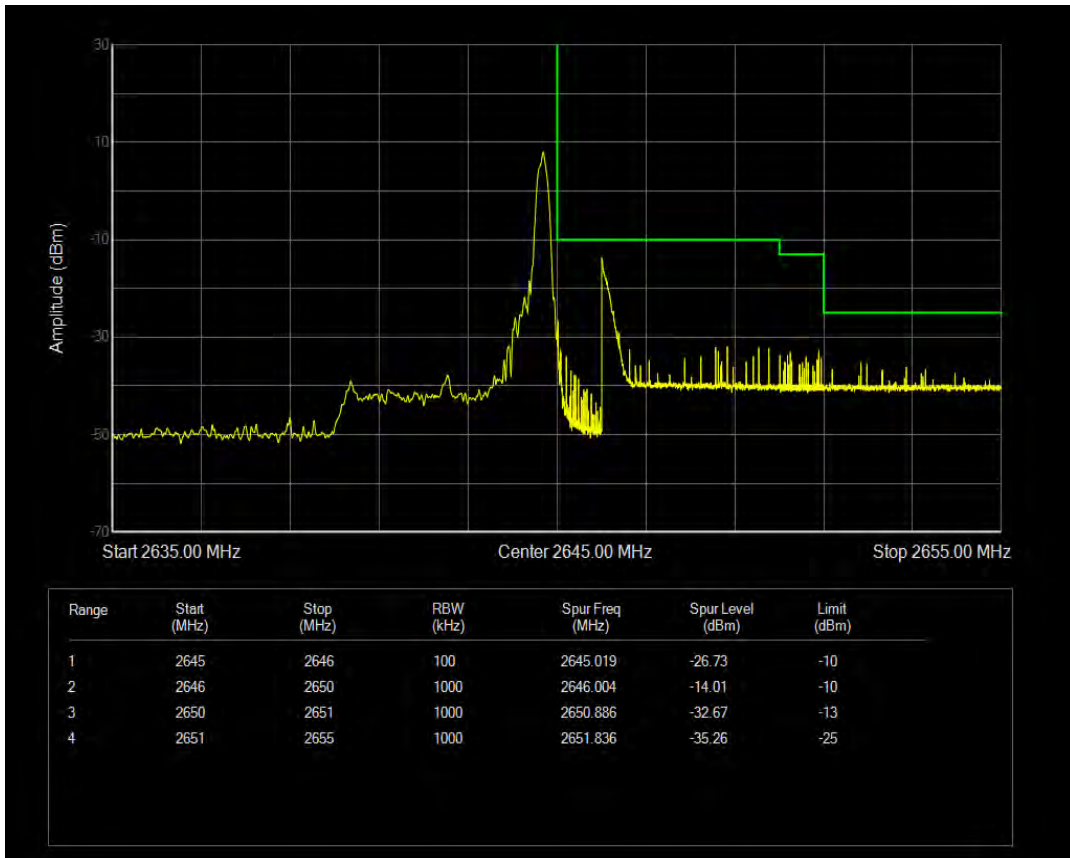
Band41 QAM16 BW=5MHz Channel=41115 RB Size=1 Position=#Max
