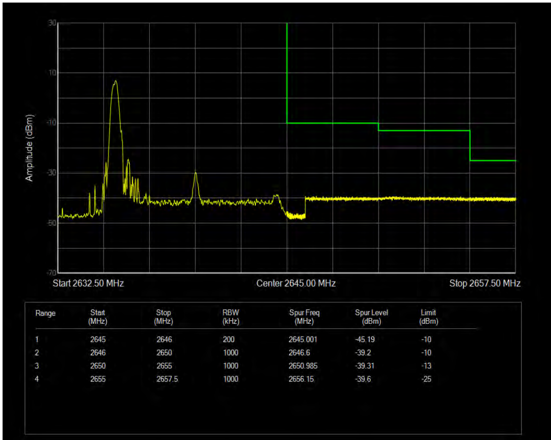
Band41 QAM16 BW=10MHz Channel=41090 RB Size=1 Position=#Max
