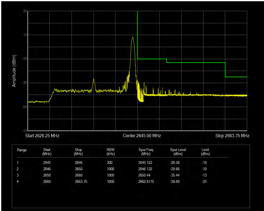
Band41 QAM16 BW=15MHz Channel=41065 RB Size=1 Position=#Max
