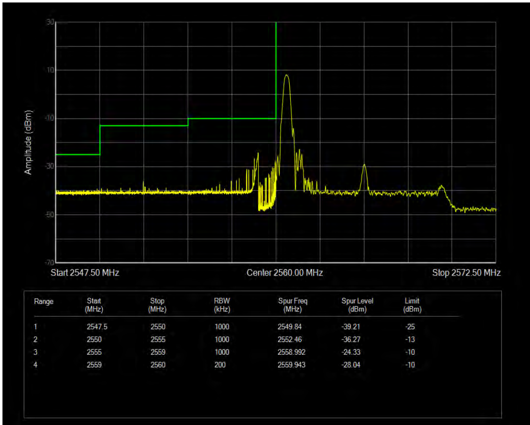
Band41 QAM16 BW=10MHz Channel=40340 RB Size=1 Position=#Max
