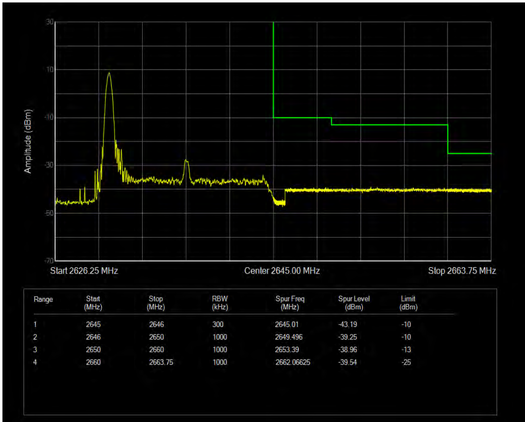
Band41 QAM16 BW=15MHz Channel=41065 RB Size=1 Position=#Max
