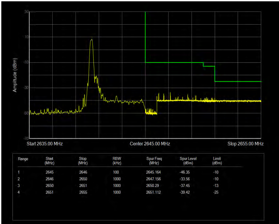
Band41 QAM16 BW=5MHz Channel=41115 RB Size=1 Position=#Max
