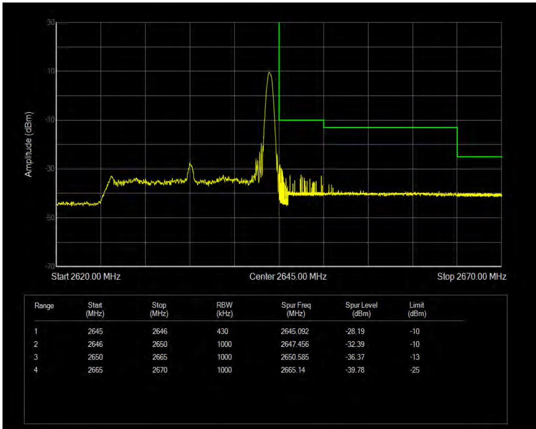
Band41 QAM16 BW=20MHz Channel=41040 RB Size=1 Position=#Max
