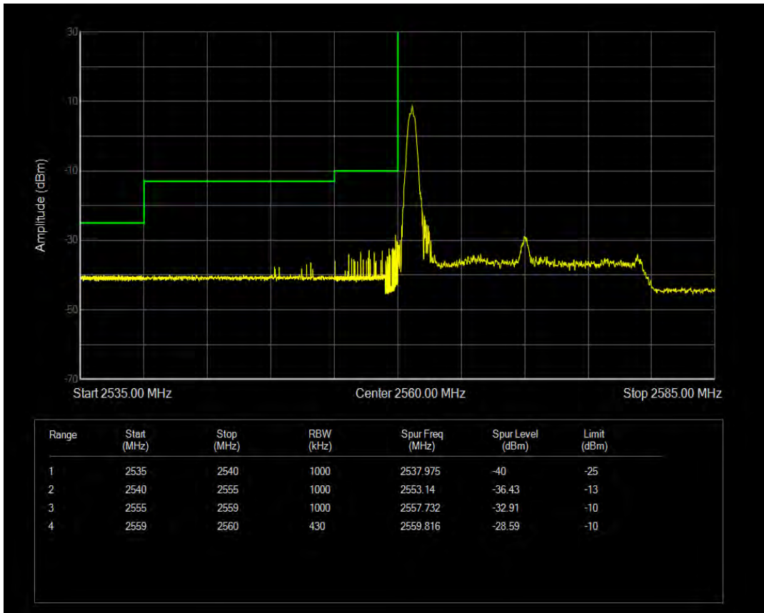
Band41 QAM16 BW=20MHz Channel=40390 RB Size=1 Position=#Max
