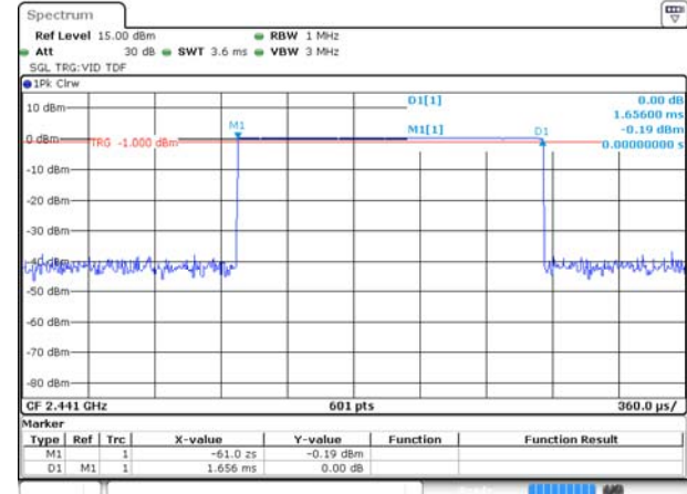
GFSK DH3
