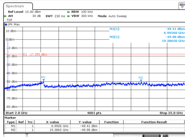
GFSK LOW CHANNEL, SPURIOUS 2 GHz ~ 25 GHz
