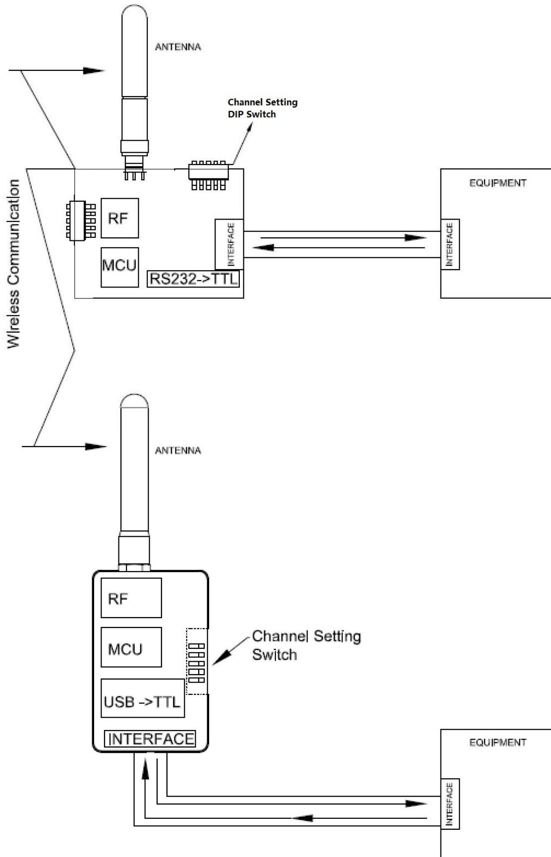
Figure 4. KTX900 Wireless Communication Application Diagram
