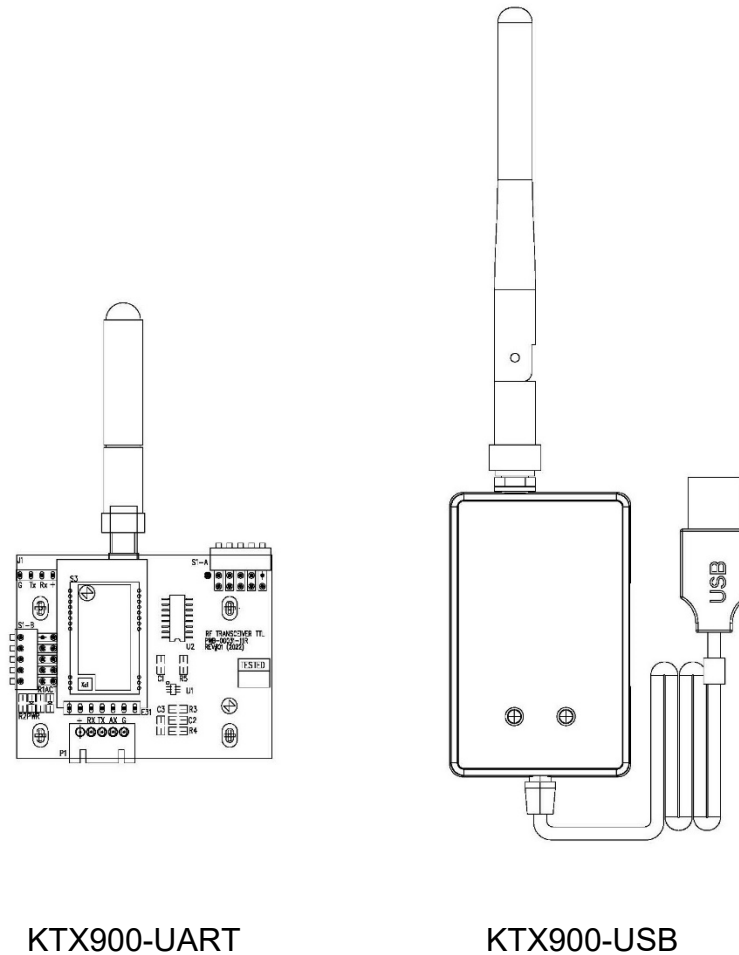
Figure 1. Wireless transceivers
