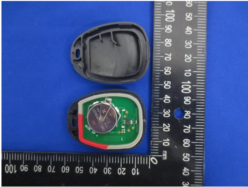
Internal photos Model: 2AOVX-3B
