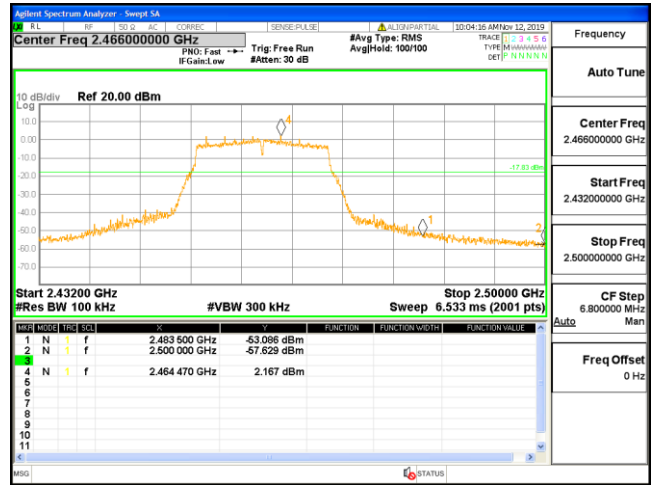
Channel 11 / 2462 MHz
