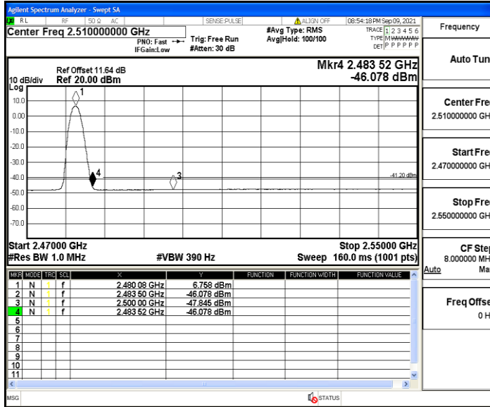
2DH5_Ant3_High_2480_Peak
