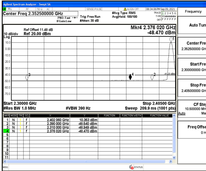
DH5_Ant3_Low_2402_Peak
