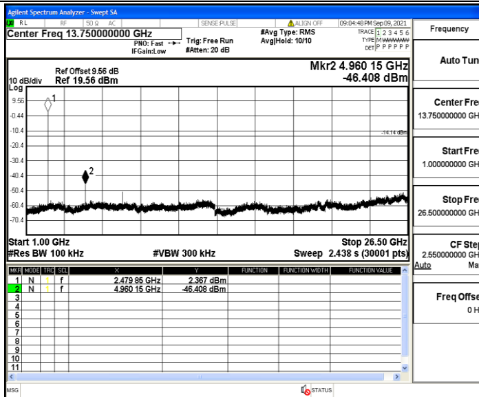
3DH5_Ant3_2480_1000~26500
