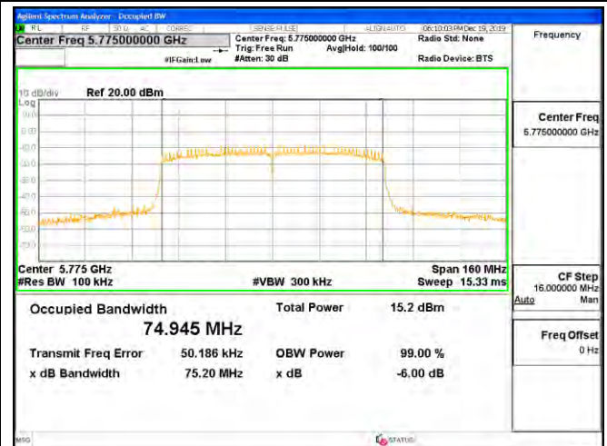
Channel 155 / 5775 MHz
