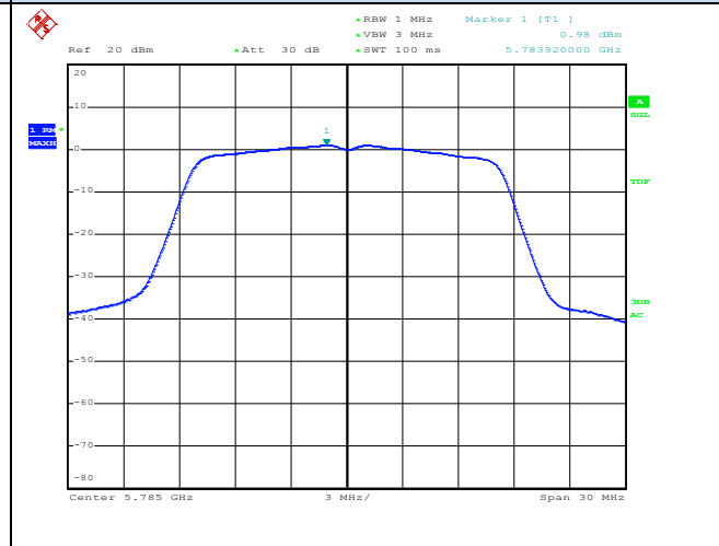
Channel 157 / 5785 MHz
