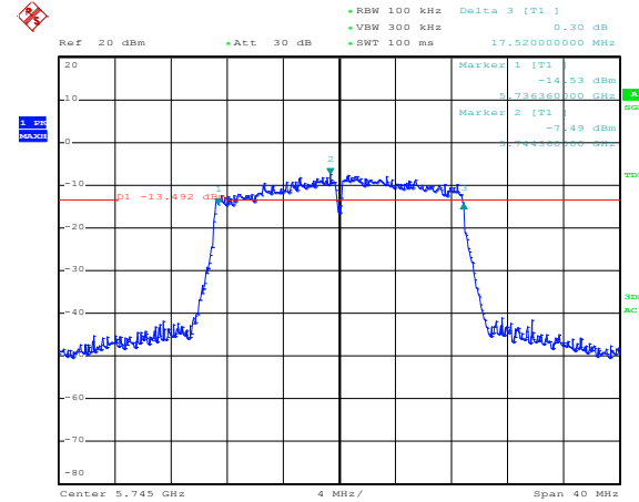
Antenna Chain 1
