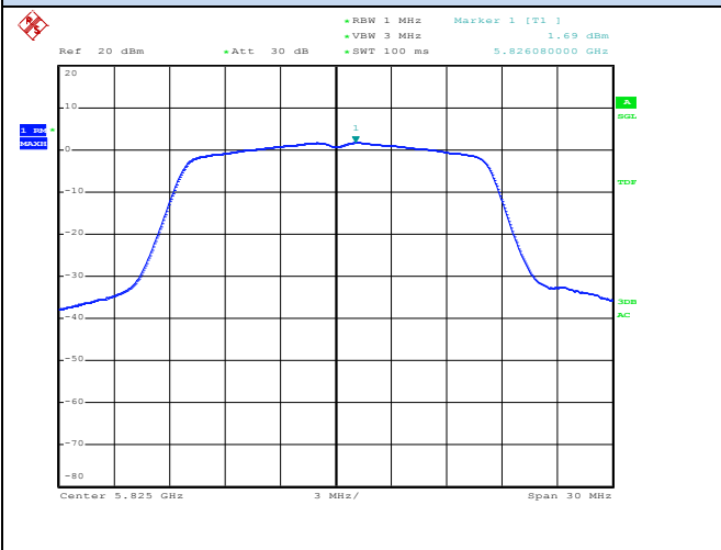
Channel 165 / 5825 MHz
