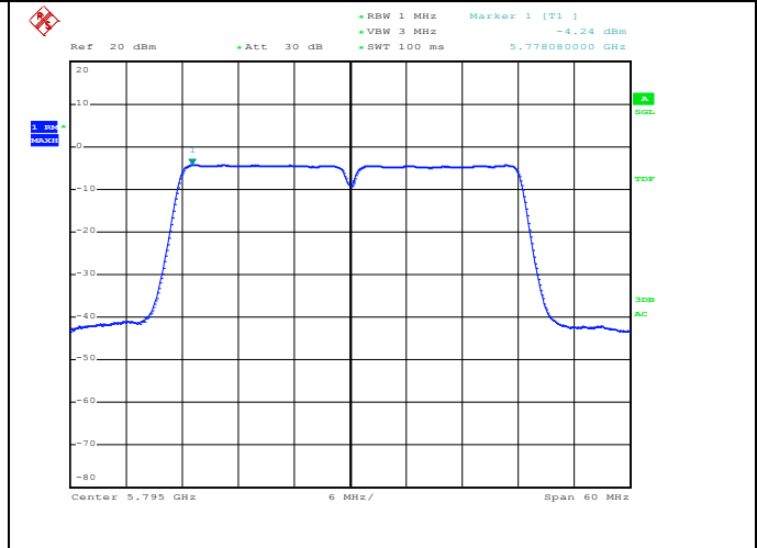
Channel 159 / 5795 MHz
