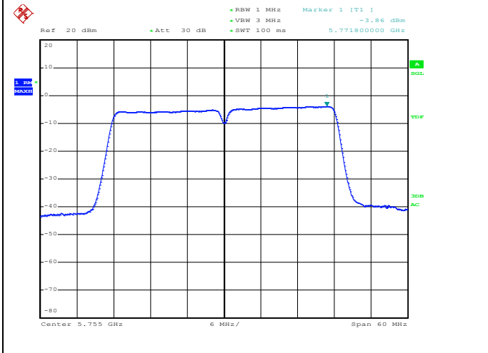
Channel 151 / 5755 MHz
