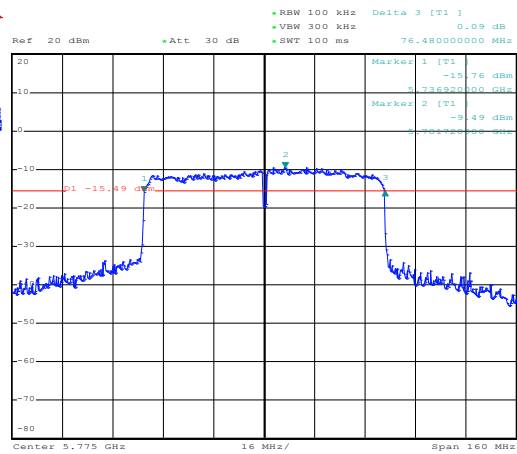
Channel 155 / 5775 MHz
