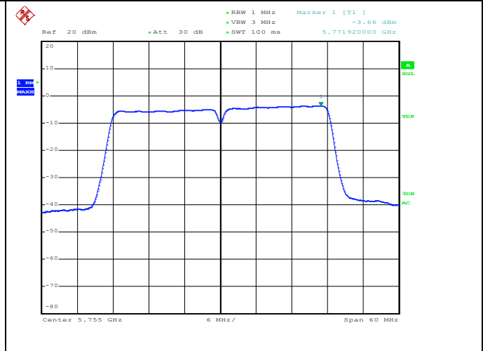
Channel 151 / 5755 MHz
