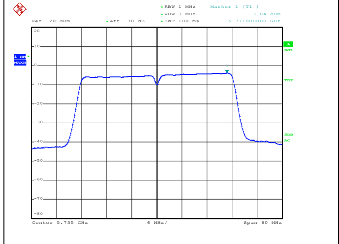
Channel 151 / 5755 MHz
