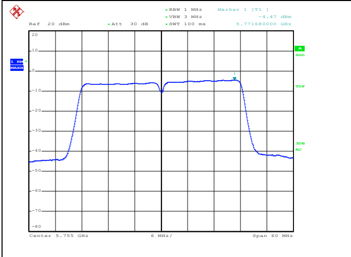
Channel 151 / 5755 MHz
