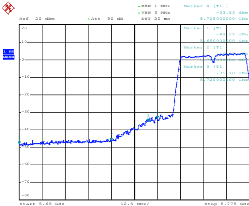
Antenna Chain 0
