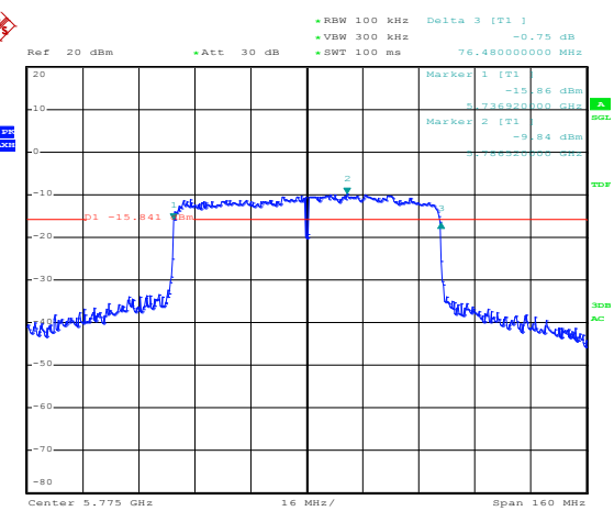
Channel 155 / 5775 MHz
