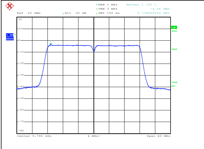
Channel 159 / 5795 MHz
