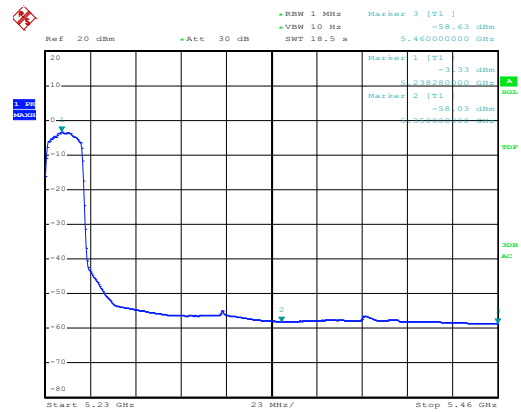
Channel 48 / 5240 MHz – Peak
