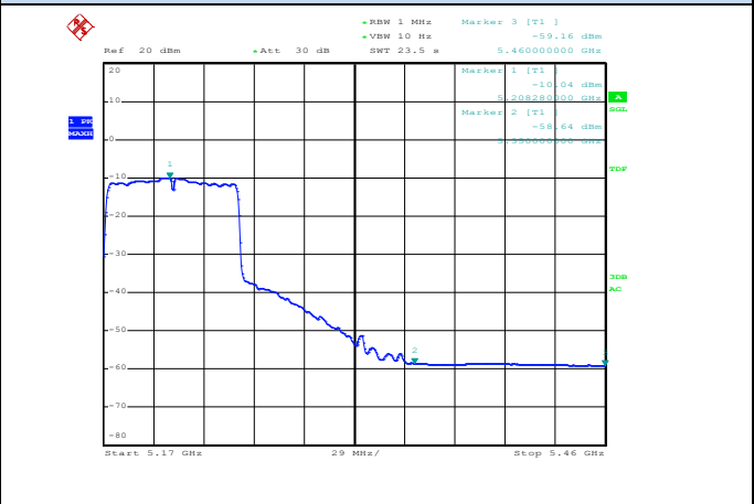
Channel 42 / 5210 MHz – Average
