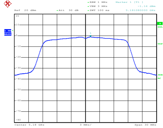
Antenna Chain 1
