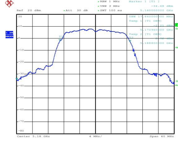
Channel 36 / 5180 MHz
