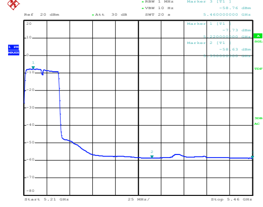
Channel 46 / 5230 MHz – Average
