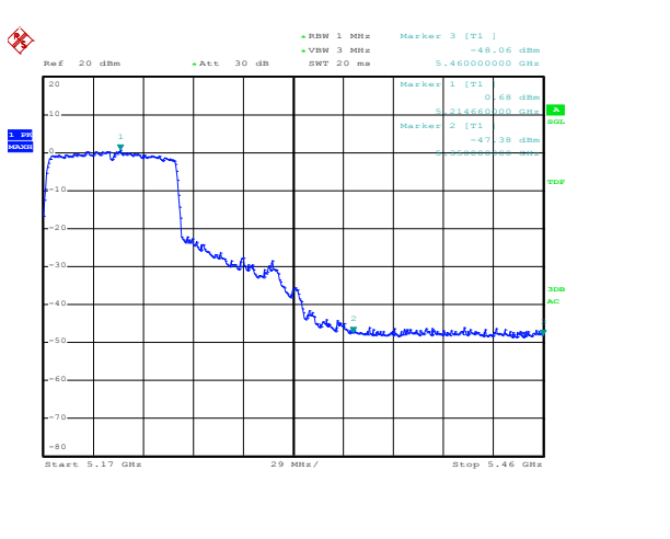
Channel 42 / 5210 MHz – Peak
