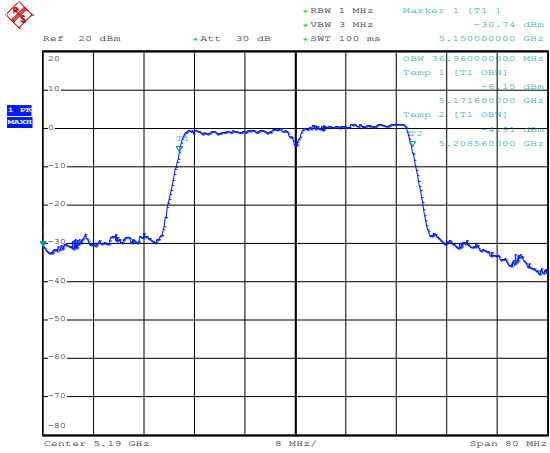
Antenna Chain 0
