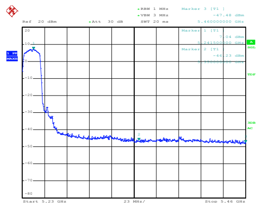
Antenna Chain 1
