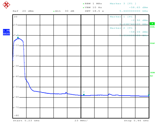
Channel 48 / 5240 MHz – Average
