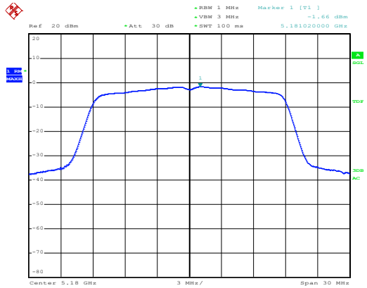
Antenna Chain 0
