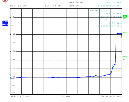
Channel 38 / 5190 MHz – Average
