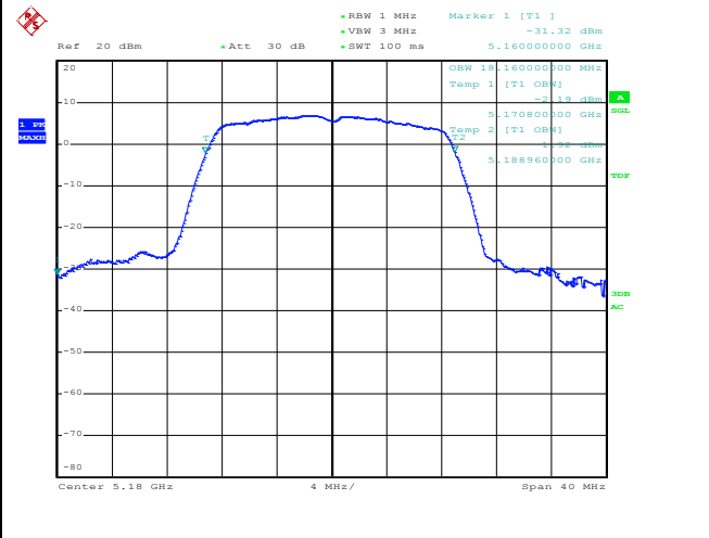
Channel 36 / 5180 MHz
