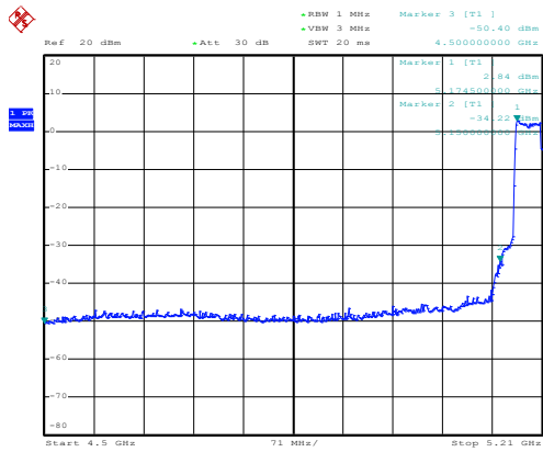
Antenna Chain 0
