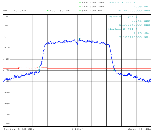
Antenna Chain 0
