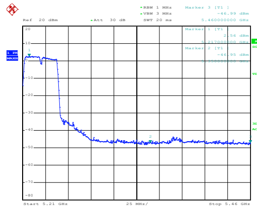
Antenna Chain 1
