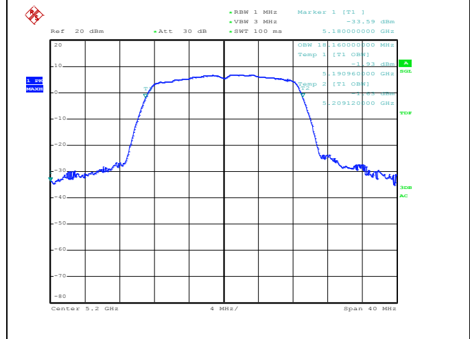
Channel 40 / 5200 MHz
