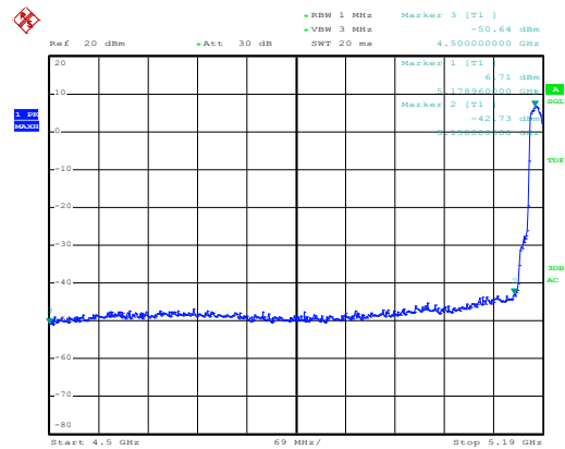
Channel 36 / 5180 MHz – Peak
