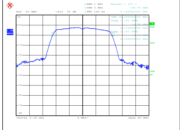
Channel 36 / 5180 MHz
