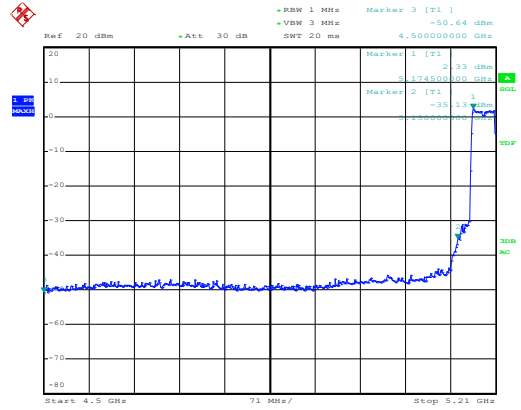
Channel 38 / 5190 MHz – Peak
