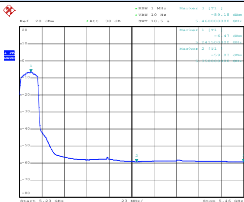
Channel 48 / 5240 MHz – Peak
