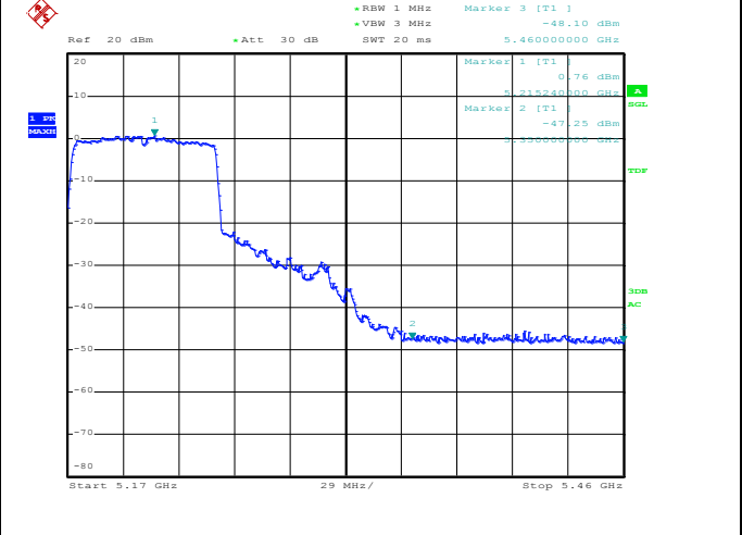
Channel 42 / 5210 MHz – Peak
