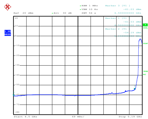
Channel 36 / 5180 MHz – Peak
