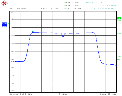
Antenna Chain 0
