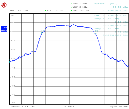
Channel 36 / 5180 MHz
