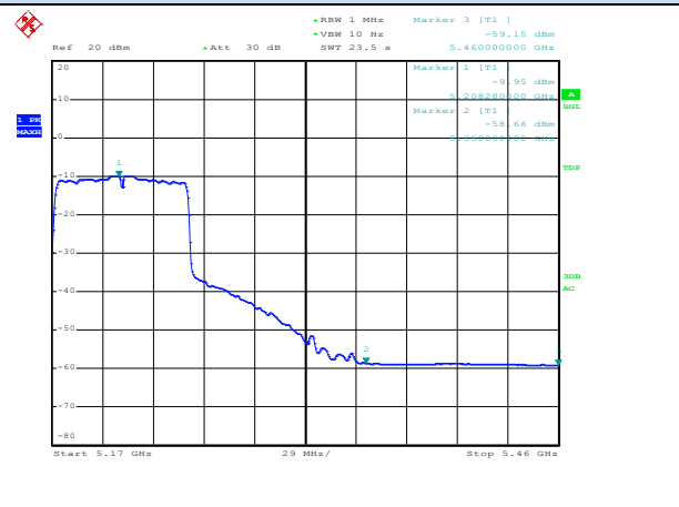
Channel 42 / 5210 MHz – Average
