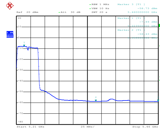
Channel 46 / 5230 MHz – Peak
