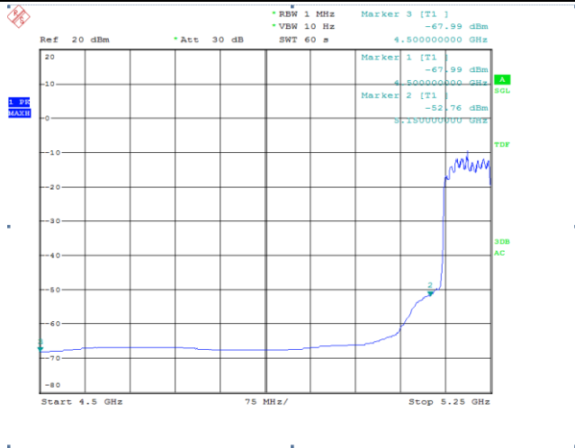
Channel 42 / 5210 MHz – Average
