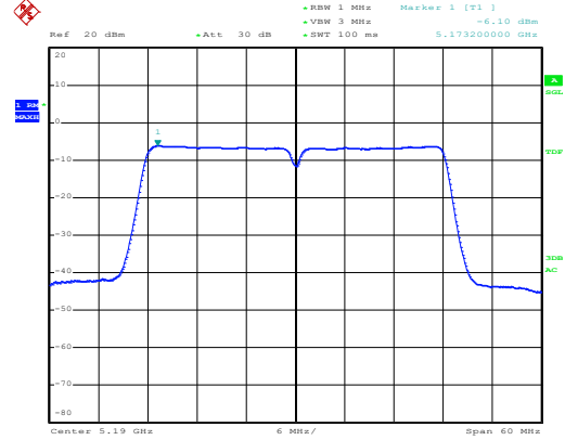
Antenna Chain 1
