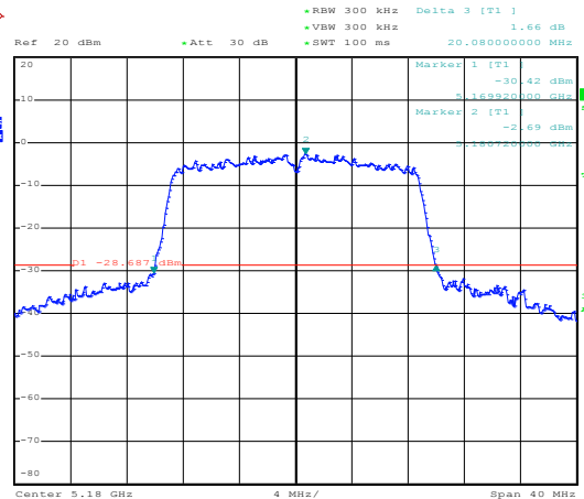
Antenna Chain 1
