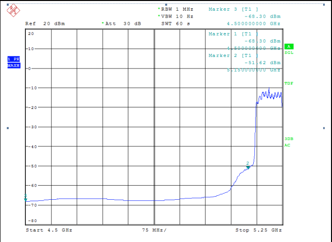
Channel 42 / 5210 MHz – Average
