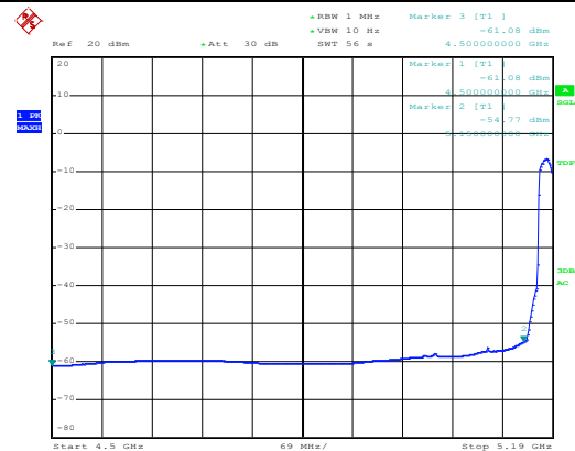
Antenna Chain 1
