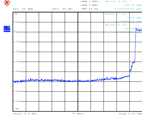
Antenna Chain 1
