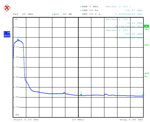
Channel 48 / 5240 MHz – Average
