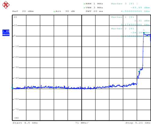
Channel 38 / 5190 MHz – Peak
