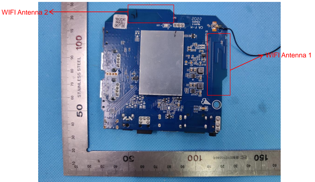
INTERNAL VIEW OF EUT (FIGURE 1)
