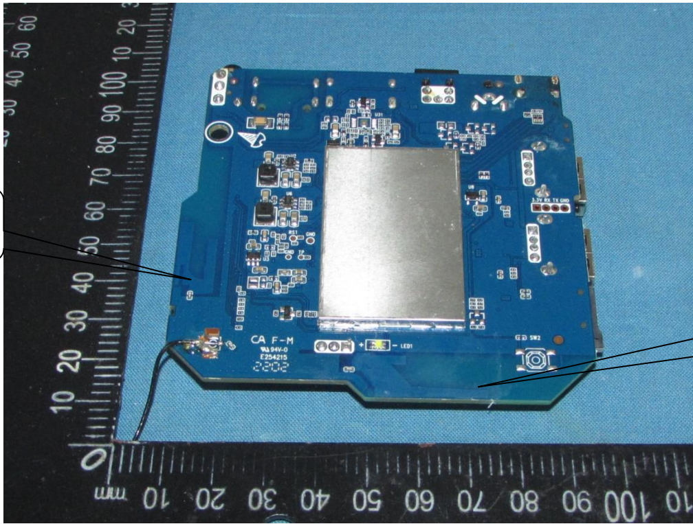
WiFi Antenna 1
