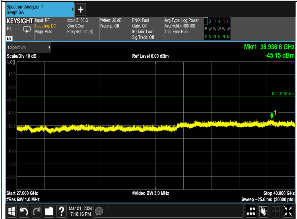
Test_Graph_802.11n40_ANT2_5795_MCS0_Frequency Band5
