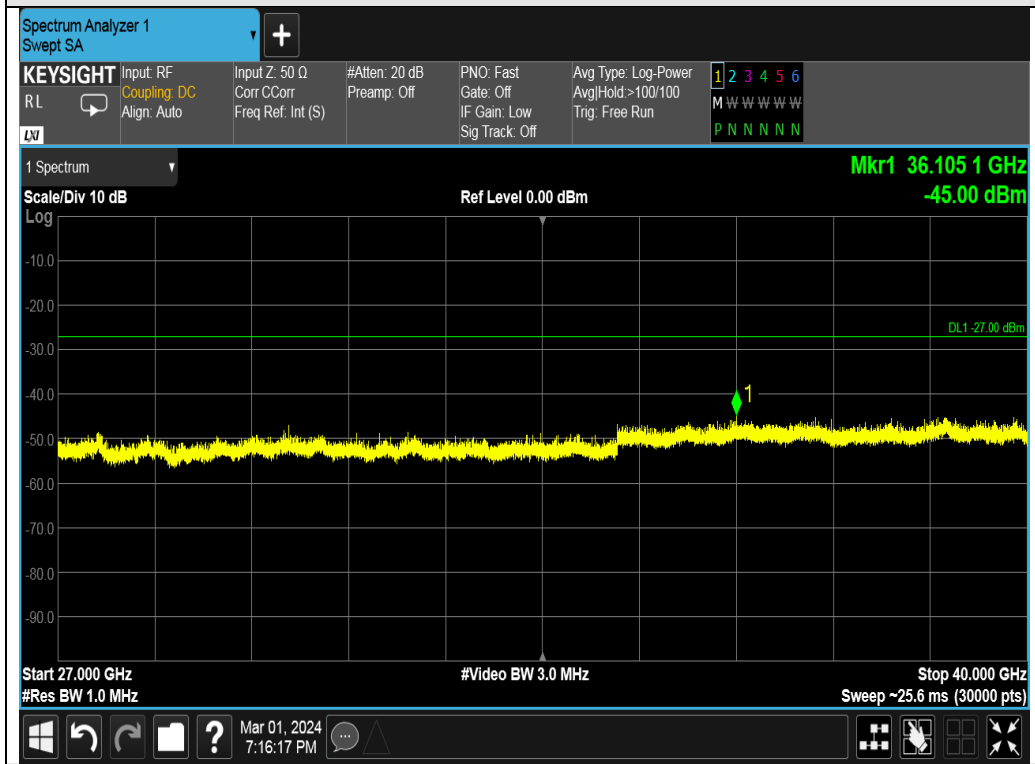
Test_Graph_802.11a_ANT2_5825_6Mbps_Frequency Band5
