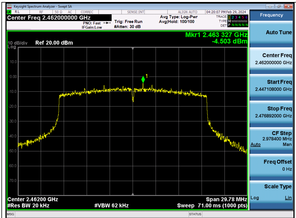
Test_Graph_802.11ax20_ANT2_2462_MCS0_PSD
