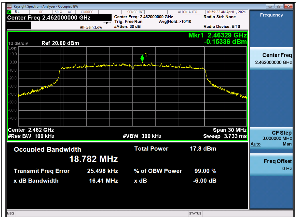
Test_Graph_802.11ax20_ANT2_2462_MCS0_DTSBW
