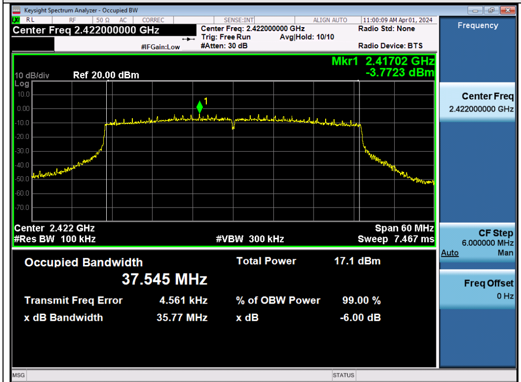
Test_Graph_802.11ax40_ANT2_2422_MCS0_DTSBW
