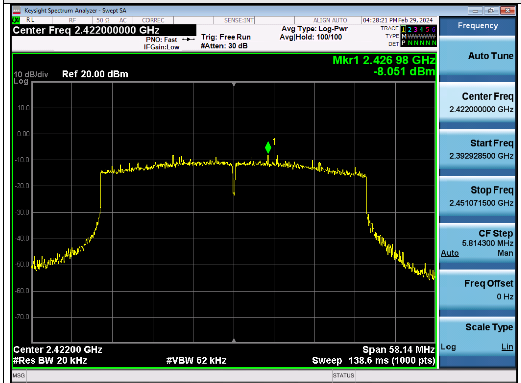
Test_Graph_802.11ax40_ANT2_2422_MCS0_PSD
