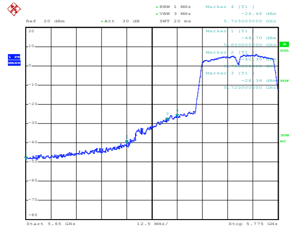
Antenna Chain 1
