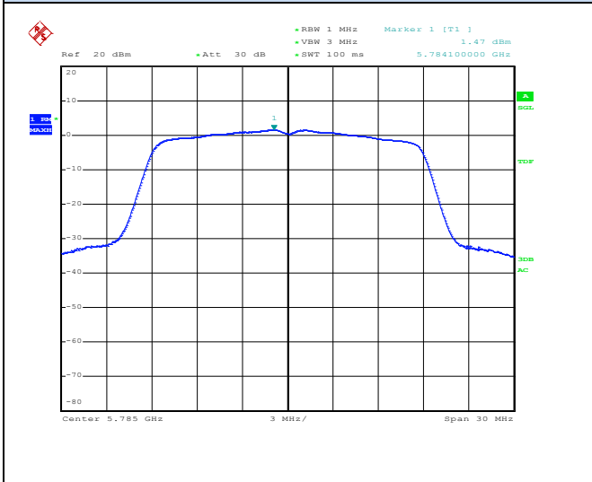
Channel 157 / 5785 MHz
