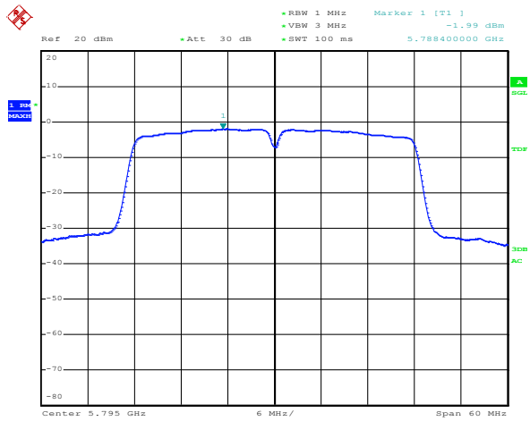
Antenna Chain 0
