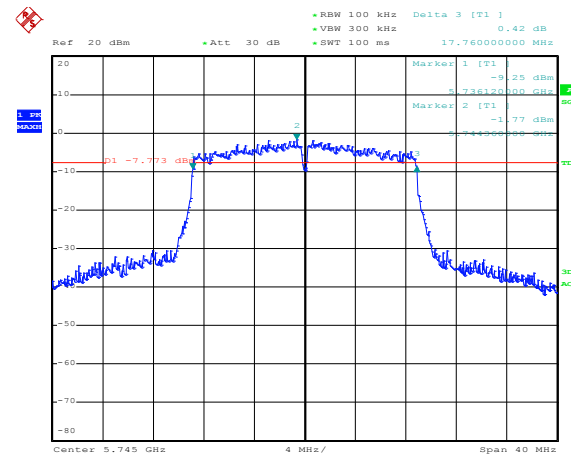
Antenna Chain 1
