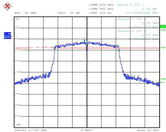
Antenna Chain 1
