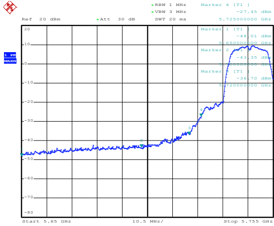
Antenna Chain 0
