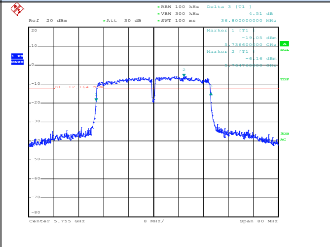
Channel 151 / 5755 MHz
