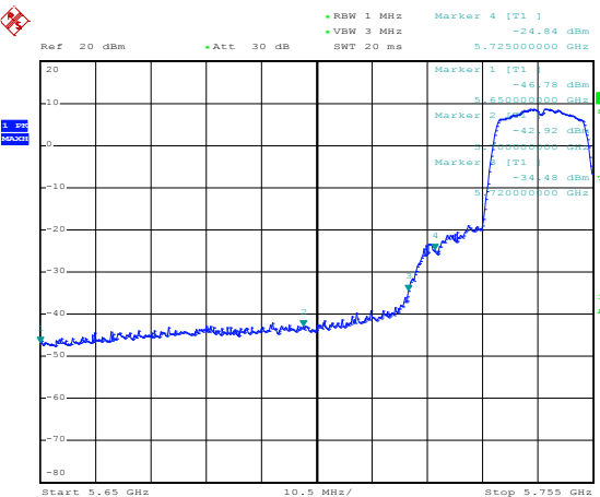
Channel 149 / 5745 MHz – Peak
