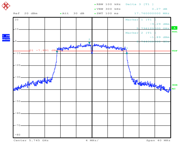
Antenna Chain 0
