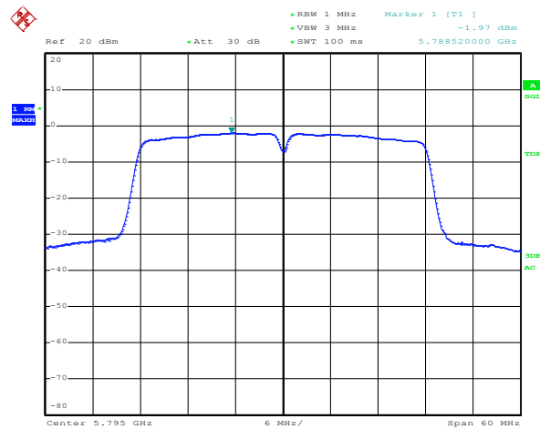
Antenna Chain 1
