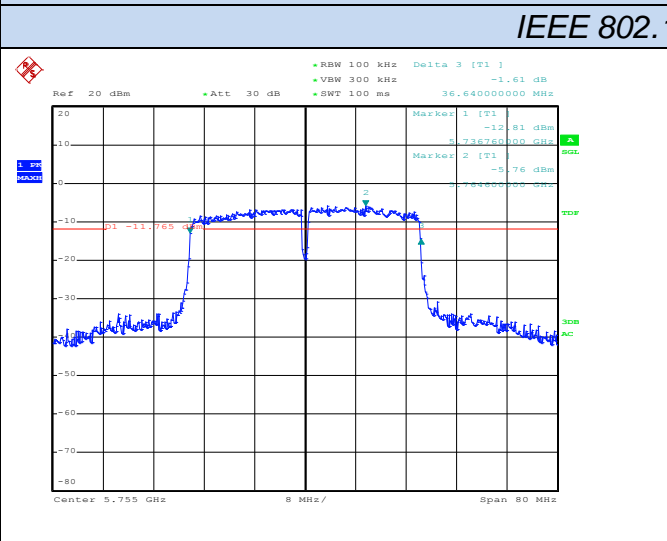
Channel 151 / 5755 MHz
