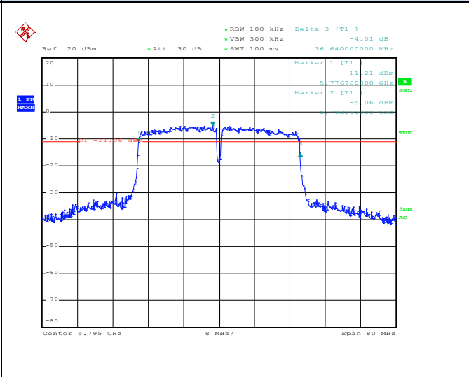
Channel 159 / 5795 MHz
