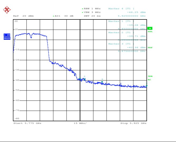
Channel 159 / 5795 MHz – Peak
