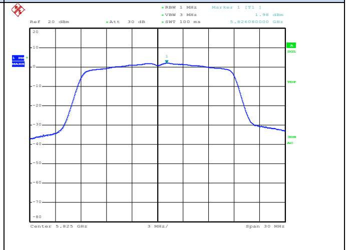
Channel 165 / 5825 MHz
