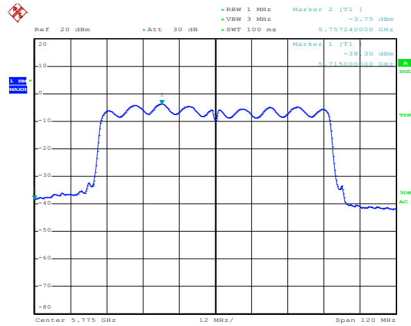
Channel 155 / 5775 MHz
