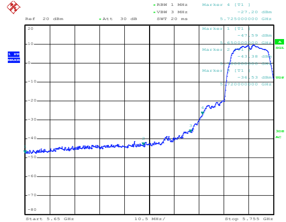
Antenna Chain 1
