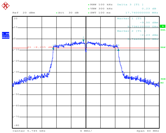
Antenna Chain 0
