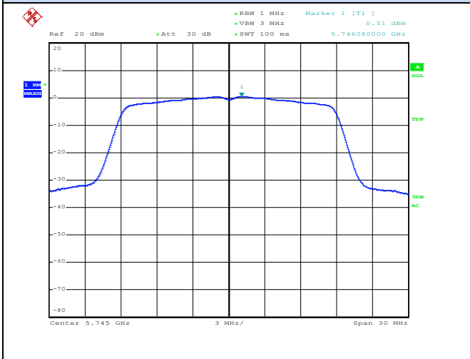
Channel 149 / 5745 MHz
