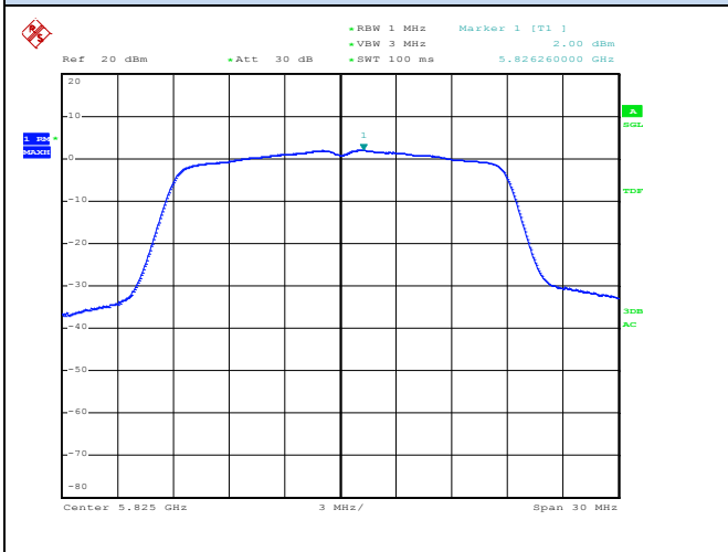
Channel 165 / 5825 MHz
