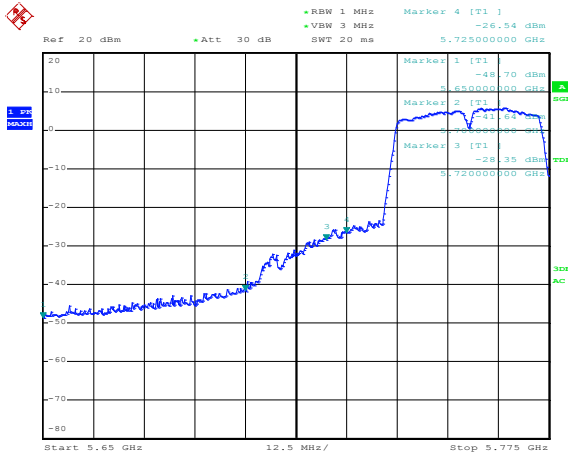
Antenna Chain 0
