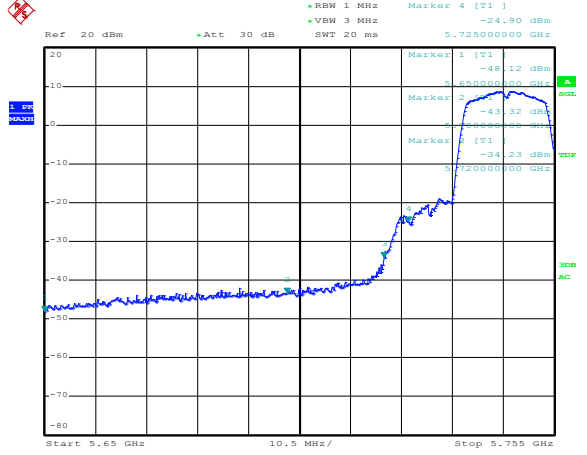
Channel 149 / 5745 MHz – Peak
