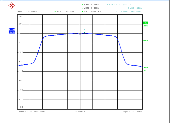
Channel 149 / 5745 MHz
