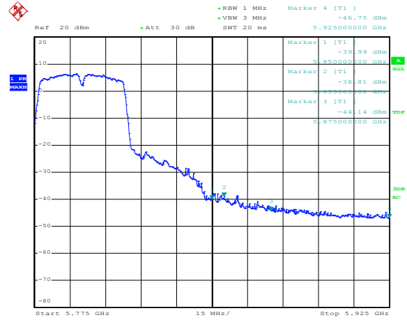
Channel 151 / 5755 MHz – Peak
