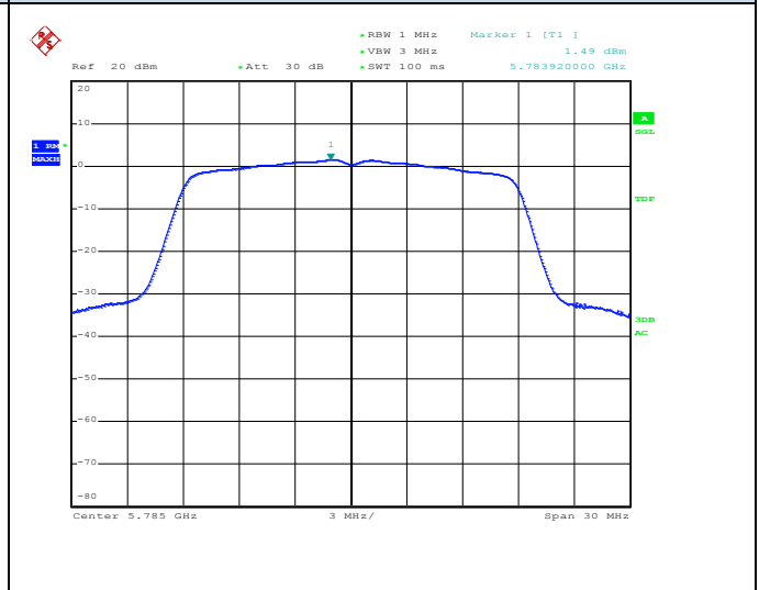
Channel 157 / 5785 MHz
