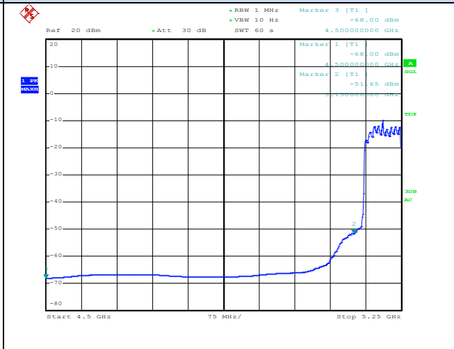
Channel 42 / 5210 MHz – Average
