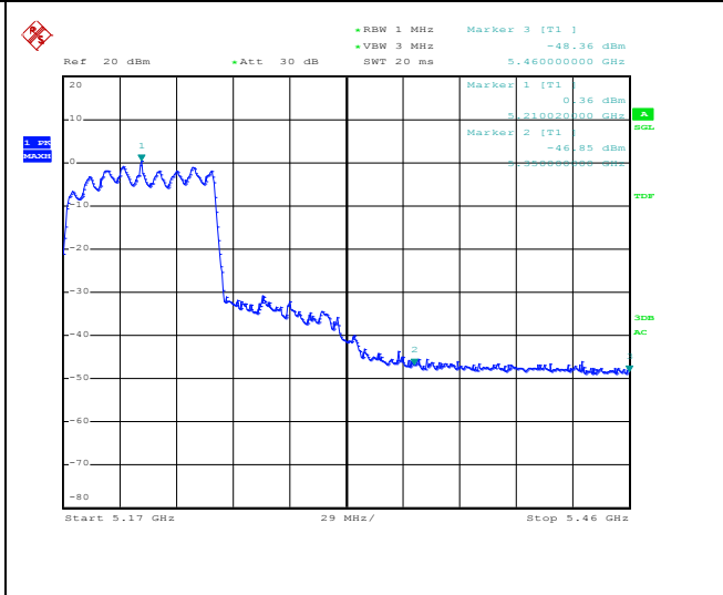
Channel 42 / 5210 MHz – Peak
