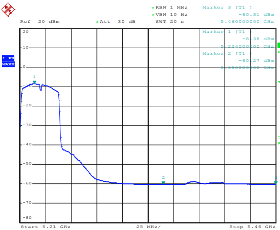
Channel 46 / 5230 MHz – Peak
