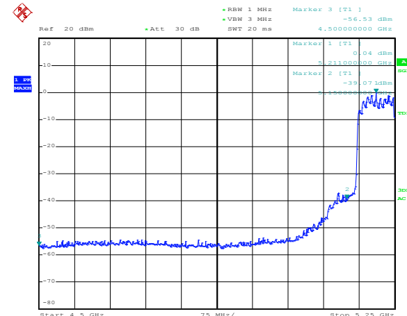
Channel 42 / 5210 MHz – Peak
