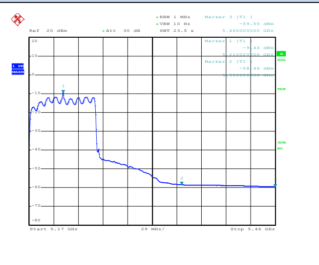
Channel 42 / 5210 MHz – Average
