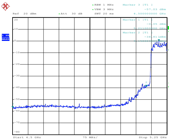
Channel 42 / 5210 MHz – Peak
