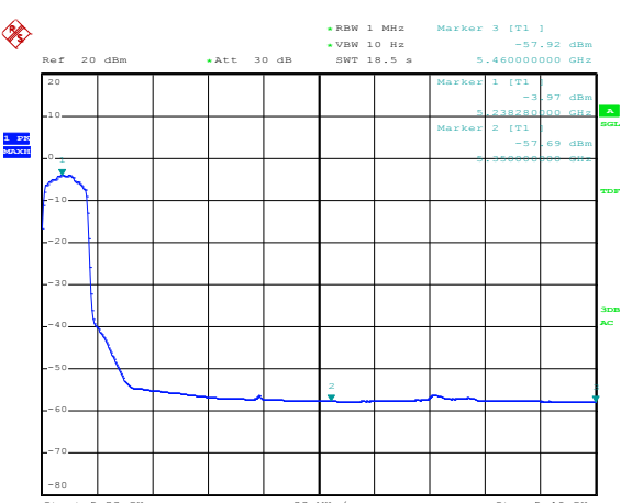
Channel 48 / 5240 MHz – Peak
