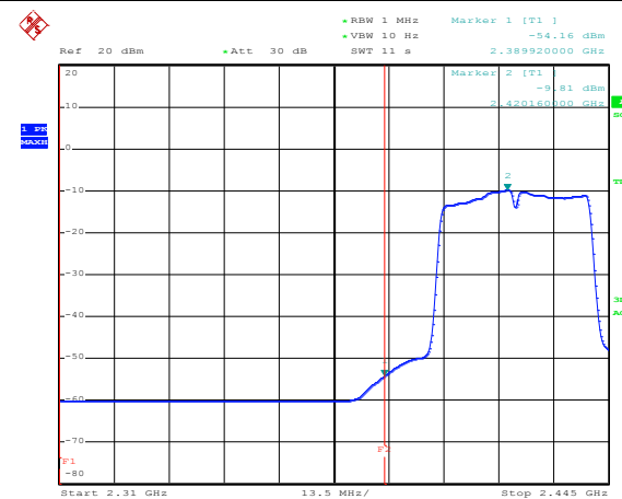
Channel 3 / 2422 MHz – Peak
