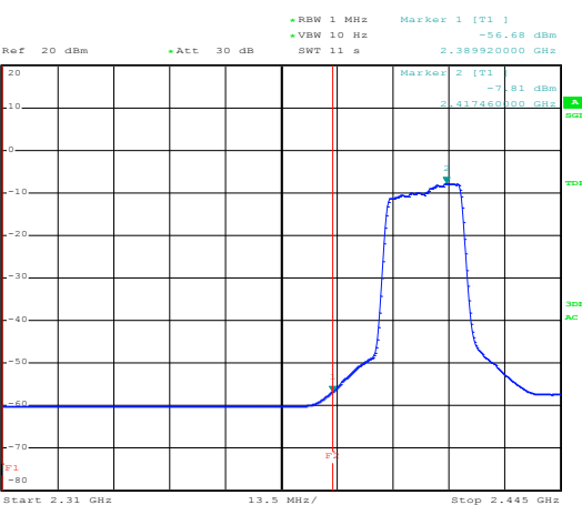
Channel 1 / 2412 MHz – Peak
