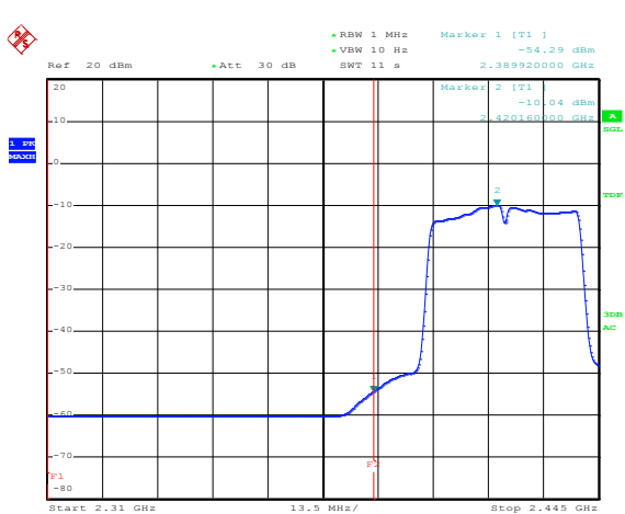
Channel 3 / 2422 MHz – Peak
