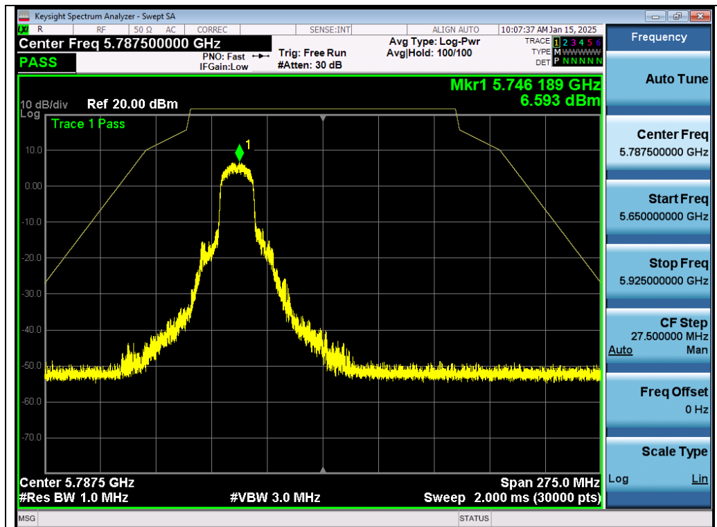
Test_Graph_802.11a_Chain B_5745_6Mbps_Frequency Band3
