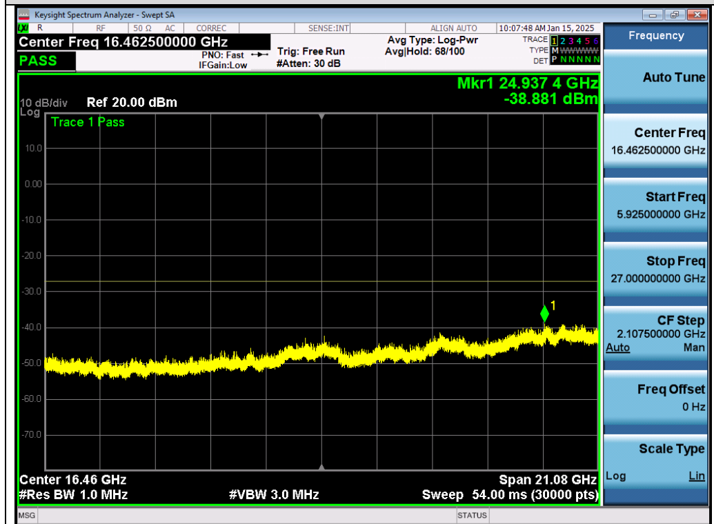
Test_Graph_802.11a_Chain B_5745_6Mbps_Frequency Band4
