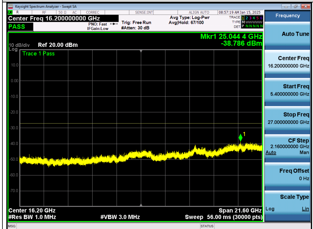
Test_Graph_802.11a_Chain B_5260_6Mbps_Frequency Band 4
