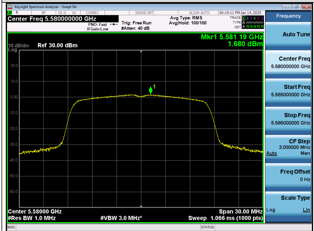
Test_Graph_802.11a_Chain A_5580_6Mbps_PSD
