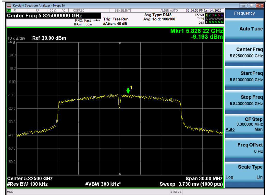
Test_Graph_802.11n20_Chain A_5825_MCS0_PSD
