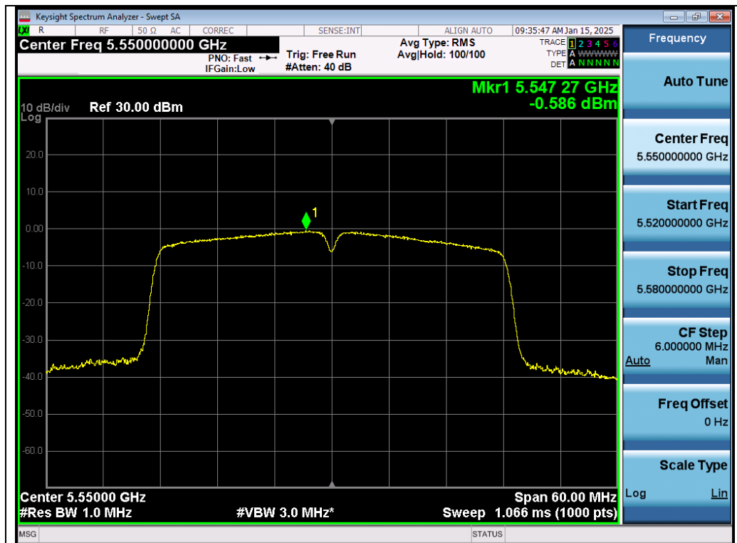
Test_Graph_802.11n40_Chain B_5550_MCS0_PSD
