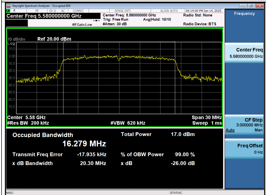
Test_Graph_802.11a_Chain A_5580_6Mbps_OBW
