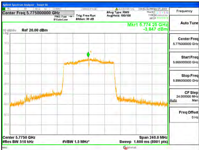
Channel 155 / 5775 MHz
