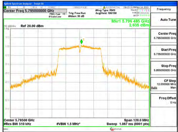
Channel 159 / 5795 MHz
