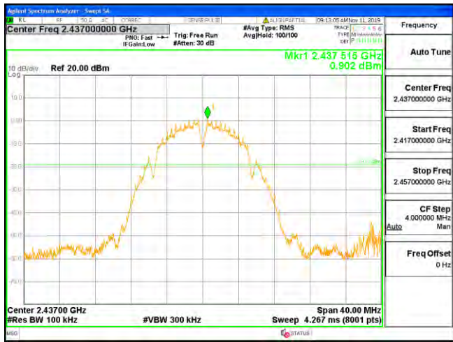
2417 MHz – 2457 MHz
