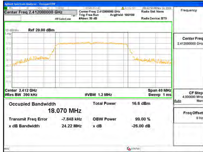
Channel 1 / 2412 MHz
