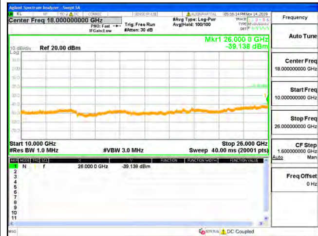
10 GHz – 26 GHz
