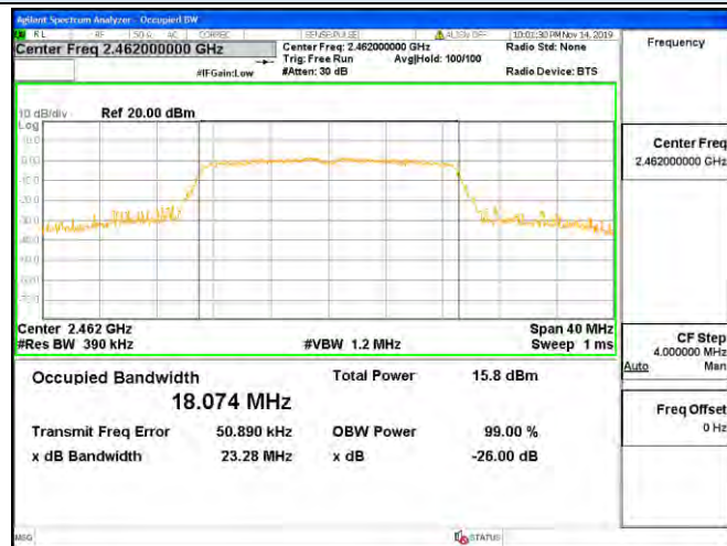
Channel 11 / 2462 MHz
