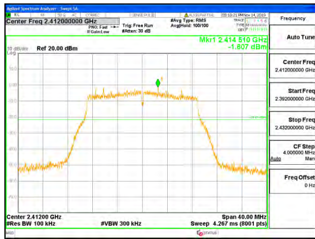
2392 MHz – 2432 MHz
