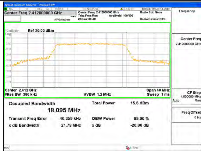
Channel 1 / 2412 MHz
