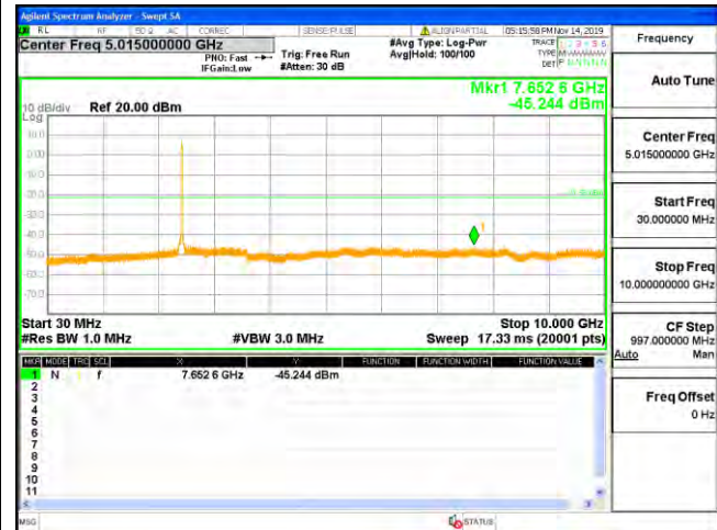
30 MHz – 10 GHz
