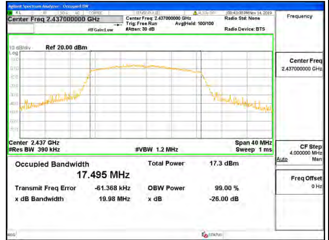
Channel 6 / 2437 MHz
