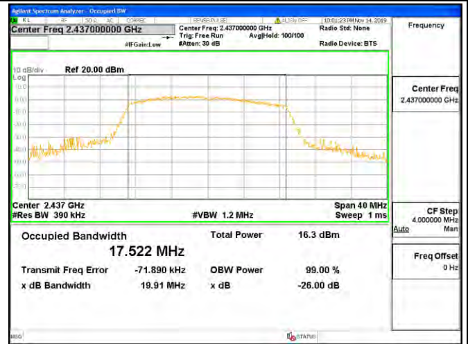
Channel 6 / 2437 MHz
