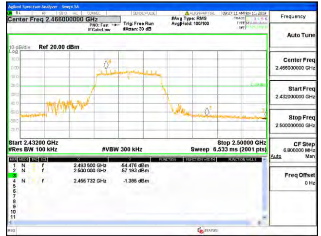
Channel 11 / 2462 MHz
