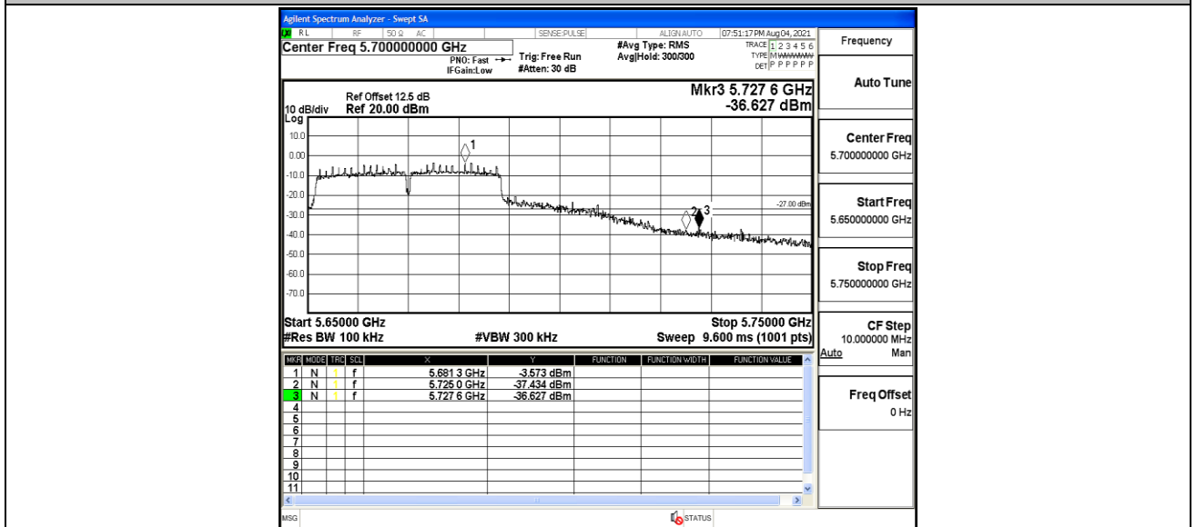
11N40MIMO_Ant2_High_5670
