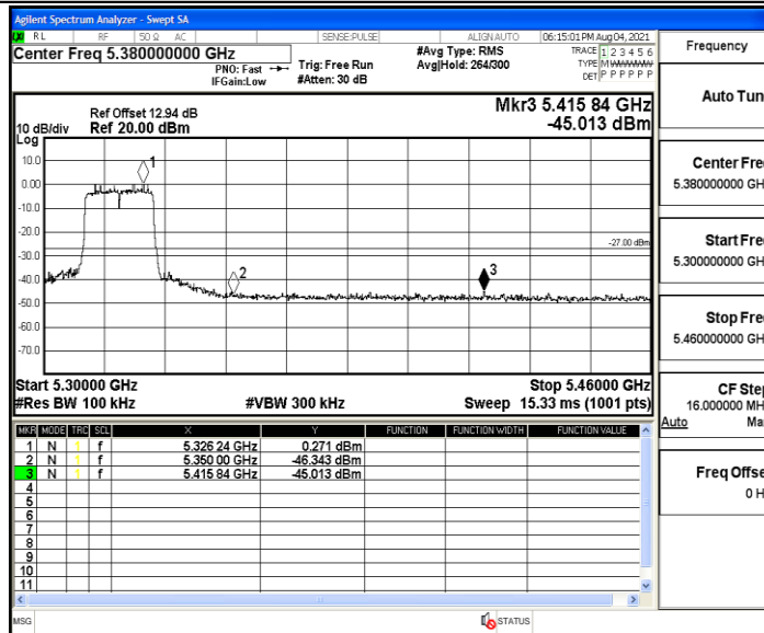
111N20MIMO_Ant1_High_5320
