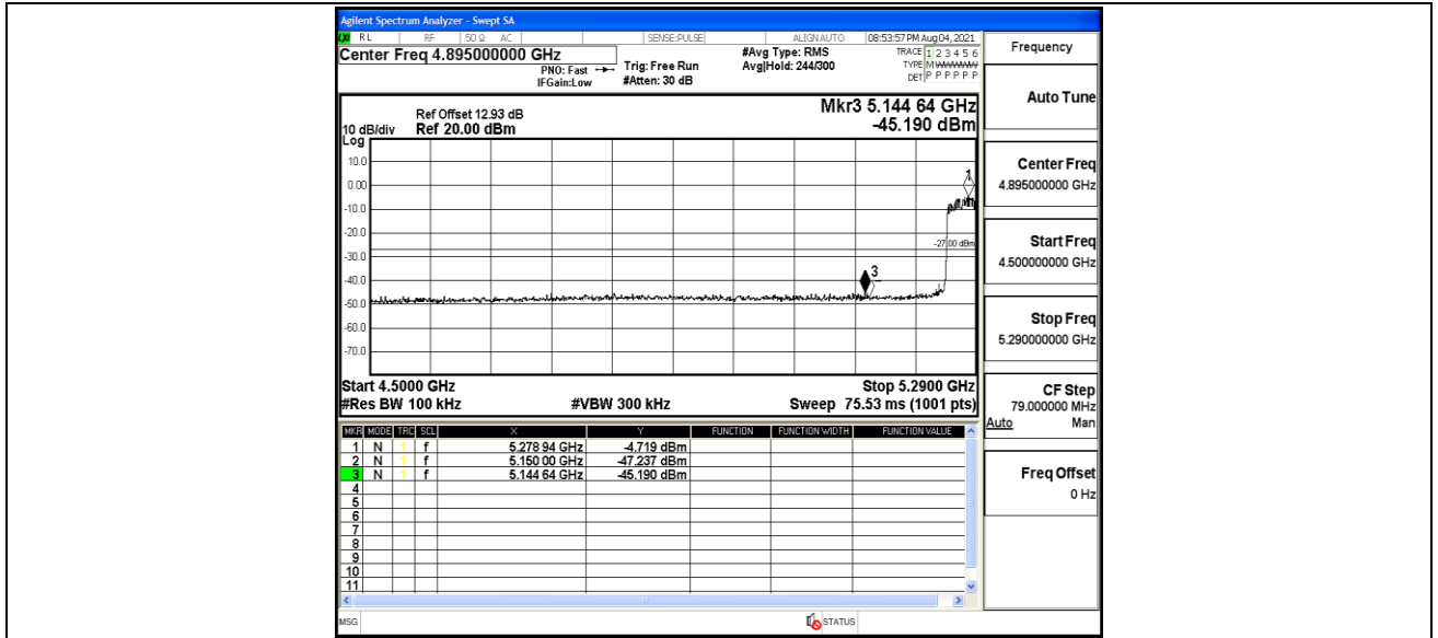
11AC40MIMO_Ant1_High_5310
