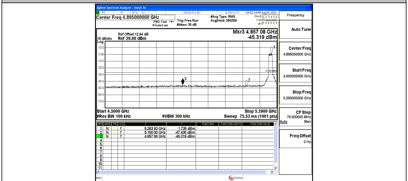
11A_Ant2_Low_5260
