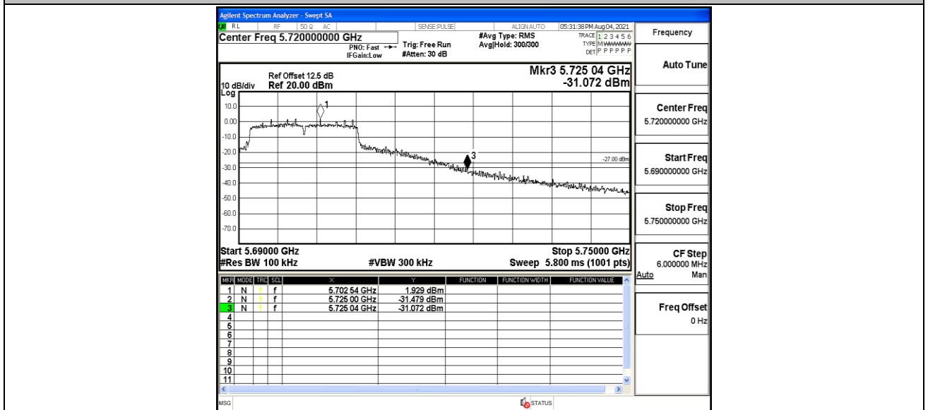
11A_Ant2_High_5700
