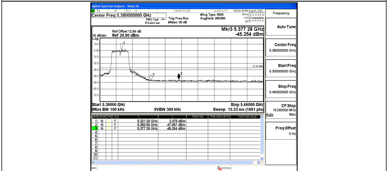
11A_Ant2_High_5320
