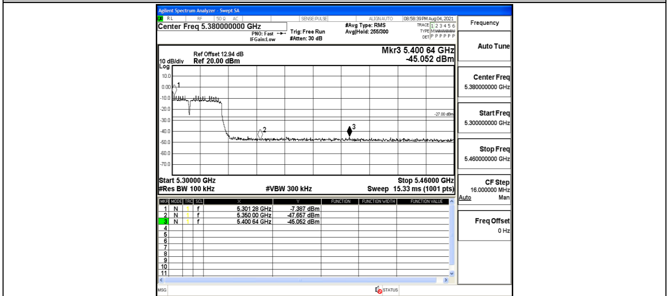
11AC40MIMO_Ant2_High_5310
