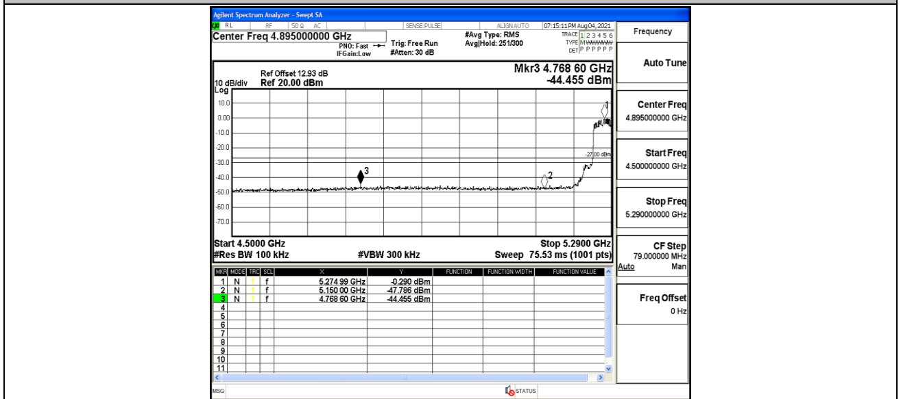
11N40MIMO_Ant1_High_5310
