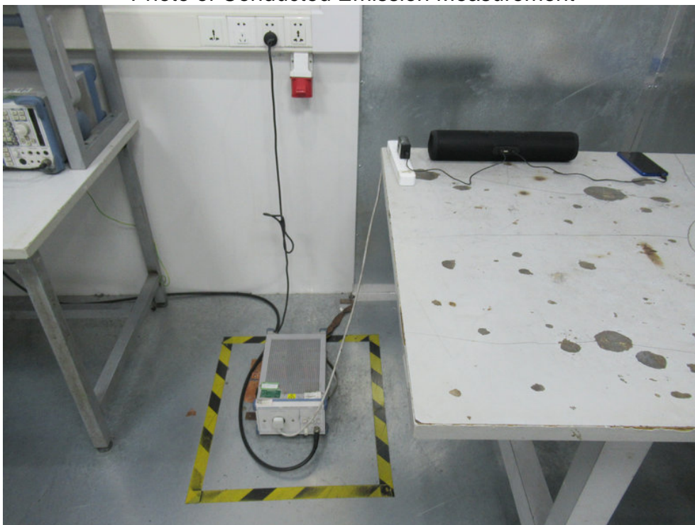
FCC ID: 2AOV6SP-055 Photo of Conducted Emission Measurement
