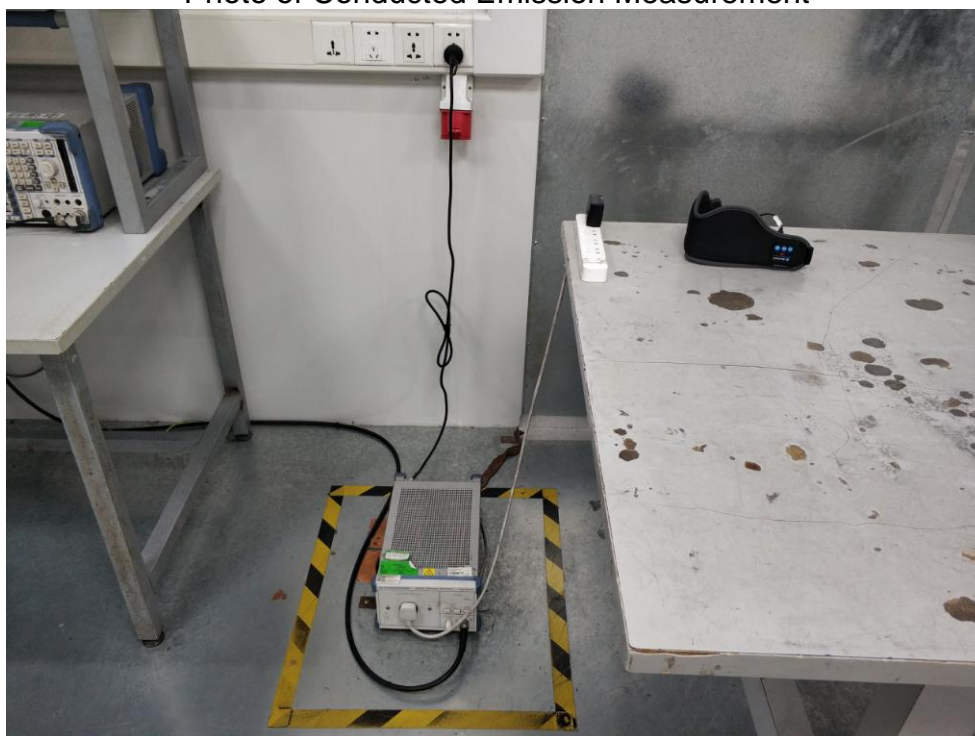
FCC ID: 2AOV6HP-092 Photo of Conducted Emission Measurement
