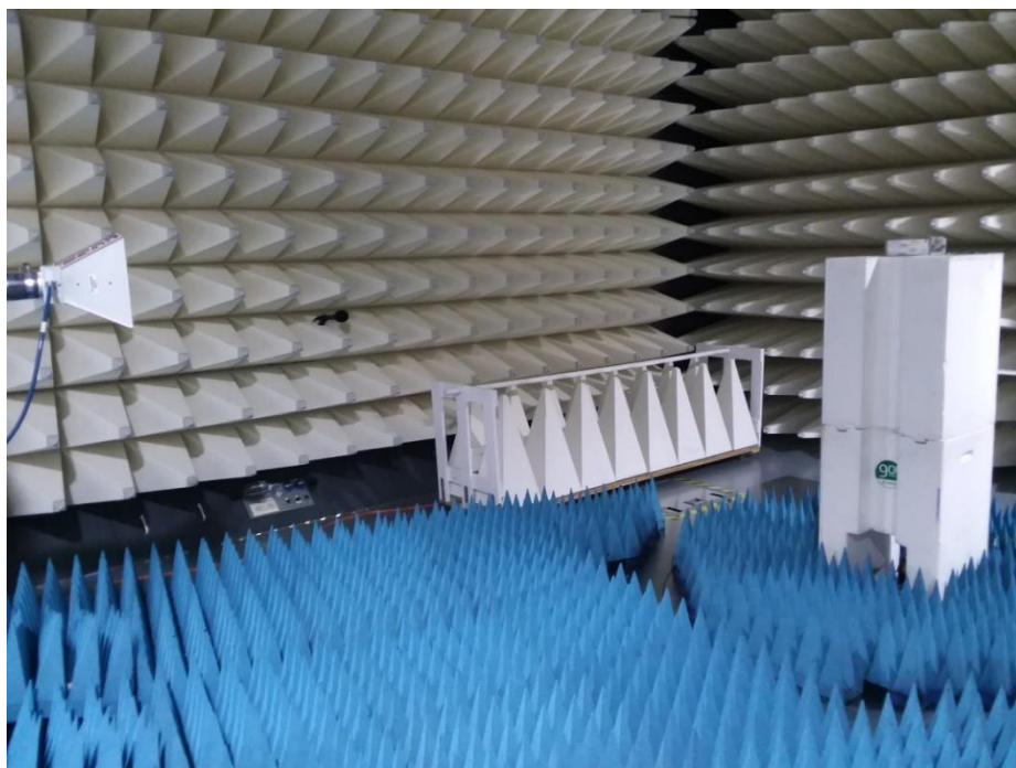
Figure C4. Radiated Emission High Range 1-18GHz test setup
