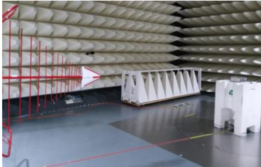
Figure C3. Radiated Emission Low Range 30-1000 MHz test setup
