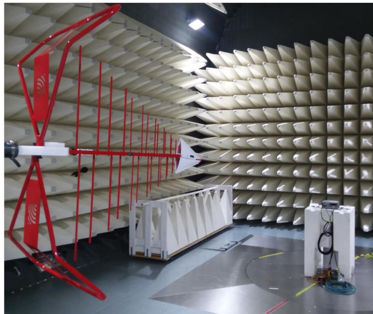
Figure B4: Radiated Emission Setup 1
