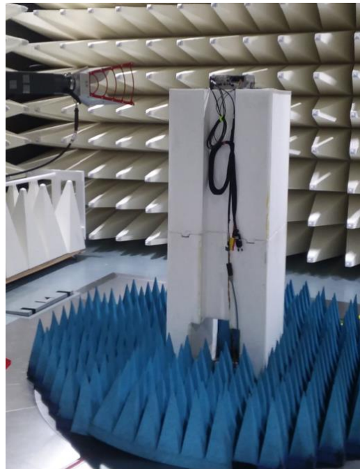
Figure B5: Radiated Emission Setup 2
