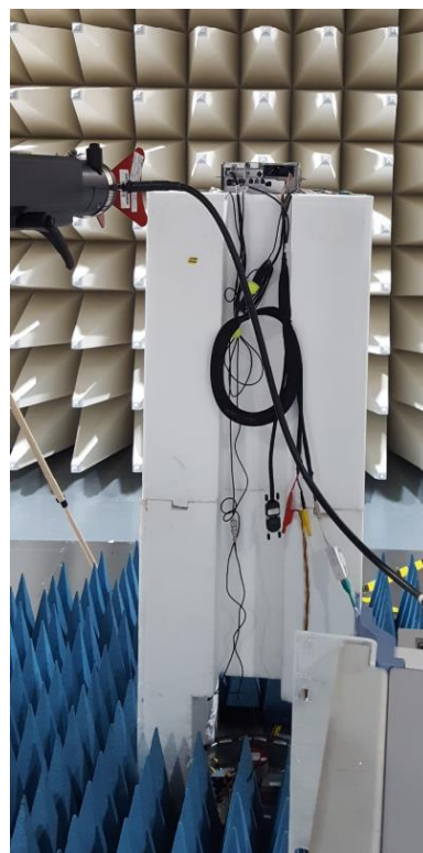
Figure B6: Radiated Emission Setup 3
