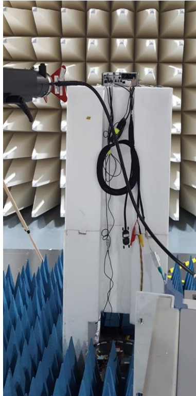
Figure D5: Radiated Emission Setup 3
