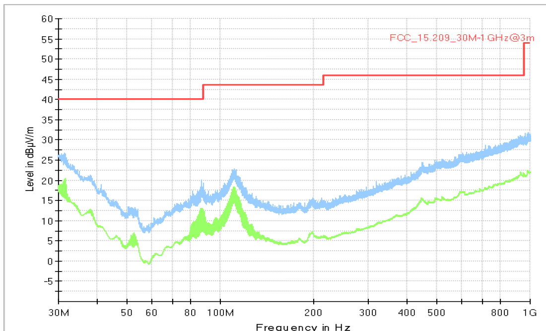
Setup_01 with immo capacitor 18 nF
