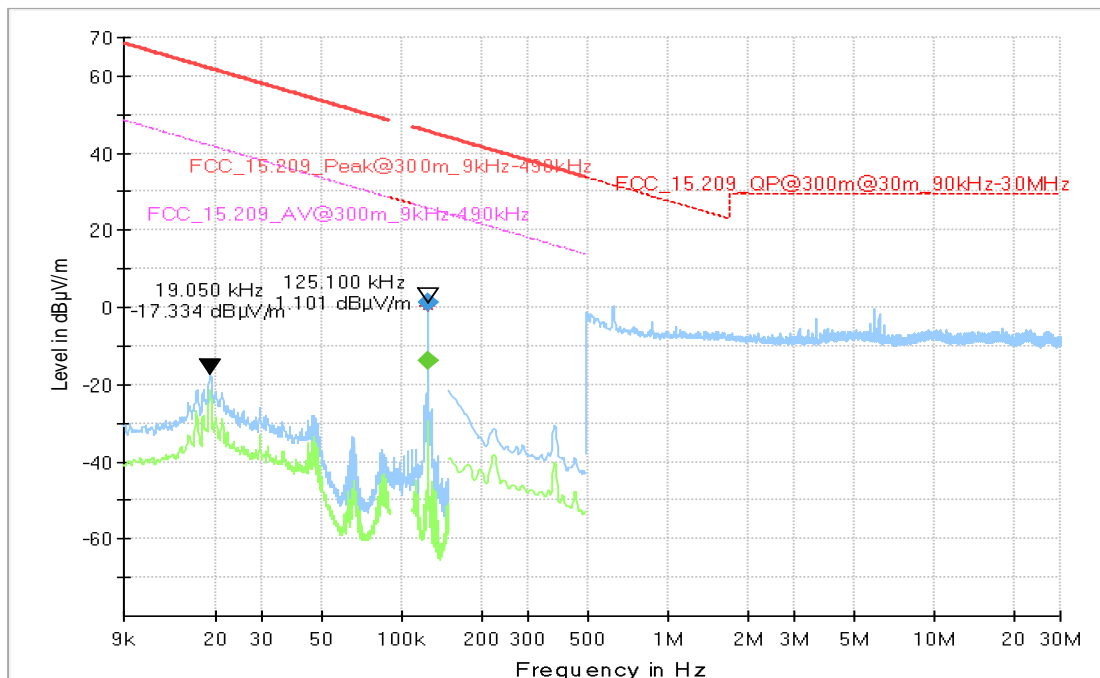
Setup_01 with immo capacitor 18 nf
