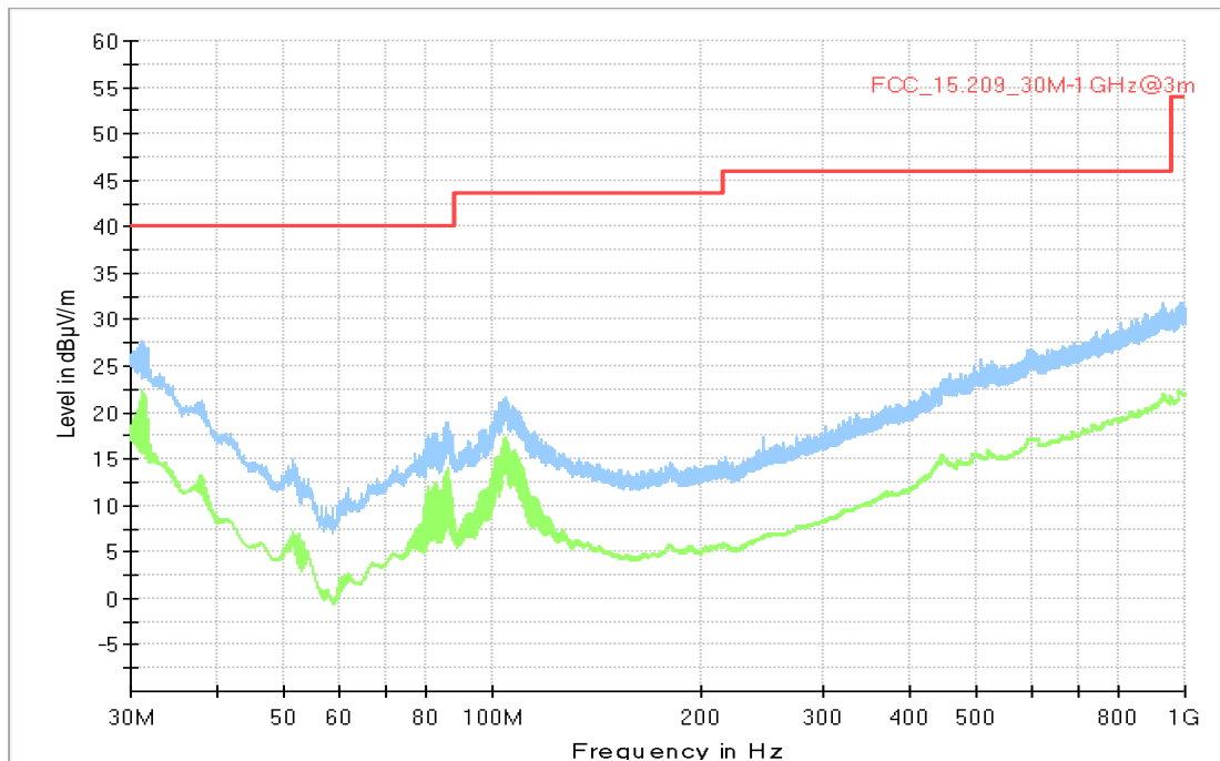
Setup_03 with immo capacitor 12 nF
