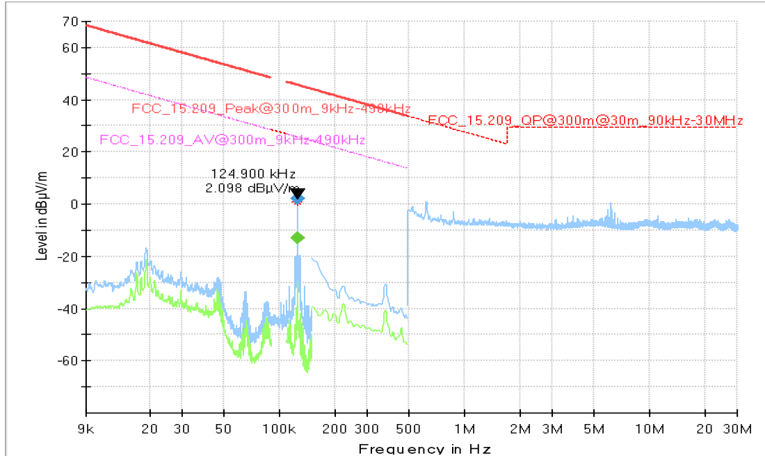
Setup_03 with immo capacitor 12 nf
