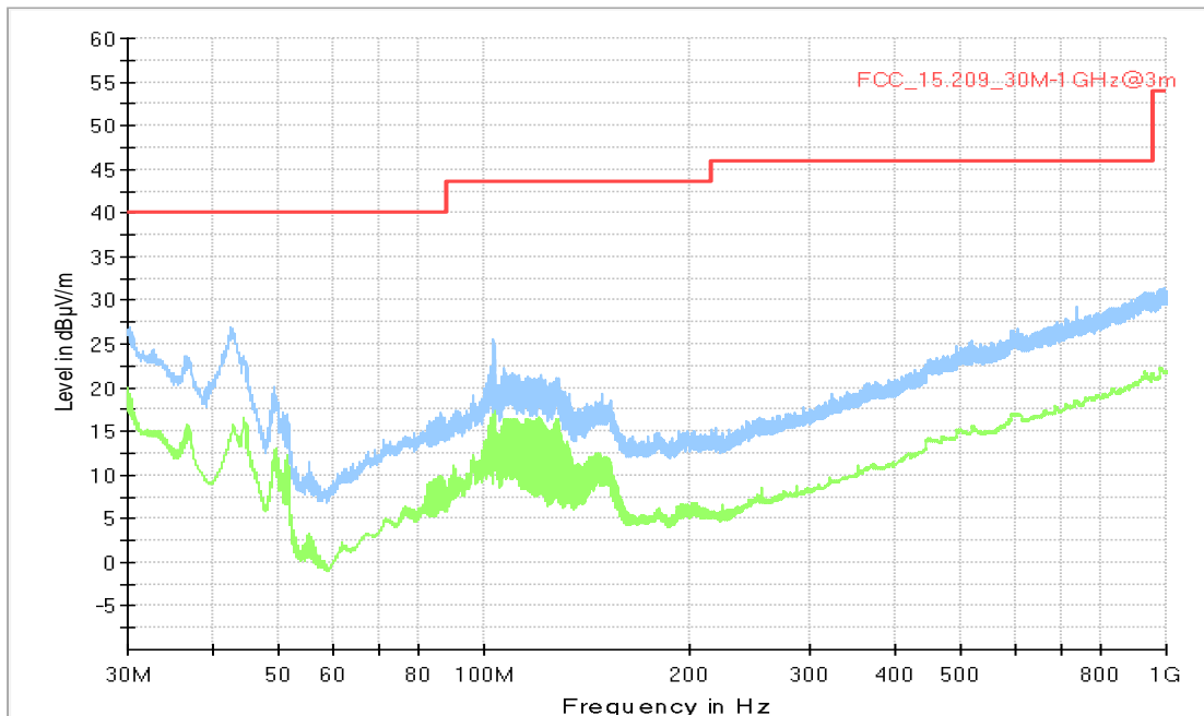
Setup_03 with immo capacitor 15 nF
