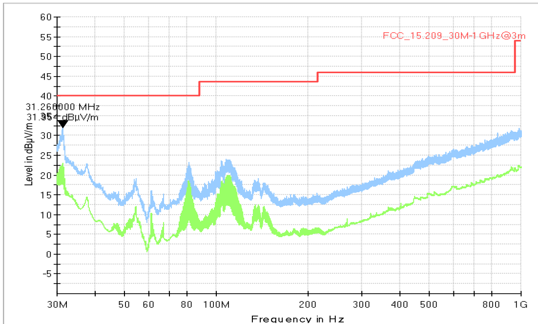
Setup_01 with immo capacitor 12 nF
