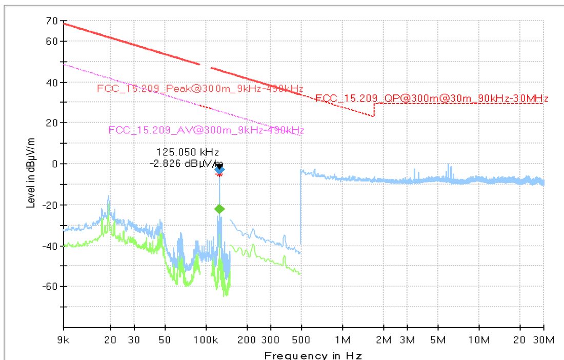
Setup_03 with immo capacitor 15 nF
