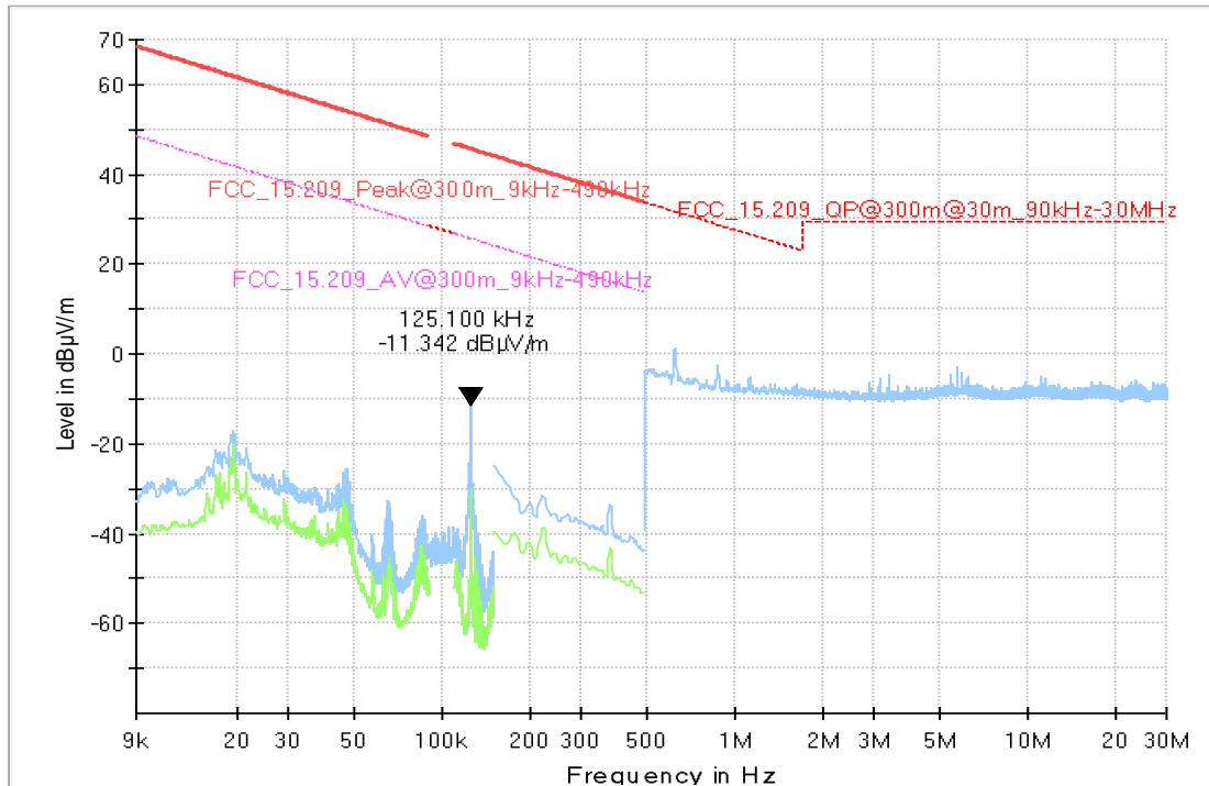
Setup_01 with immo capacitor 12 nF + Stepper motor
