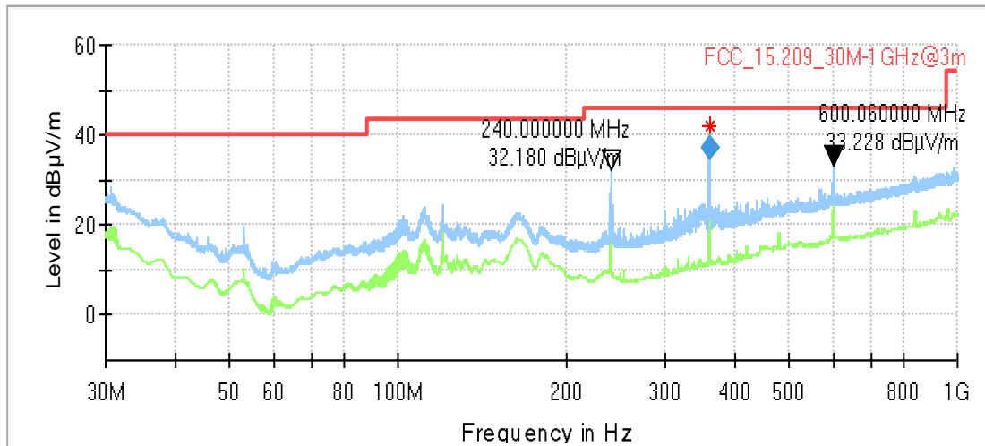
Setup_03 with immo capacitor 15 nF + Stepper motor
