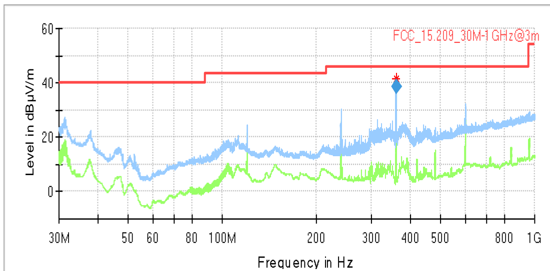
Setup_04 with immo capacitor 15 nF + Bargraph
