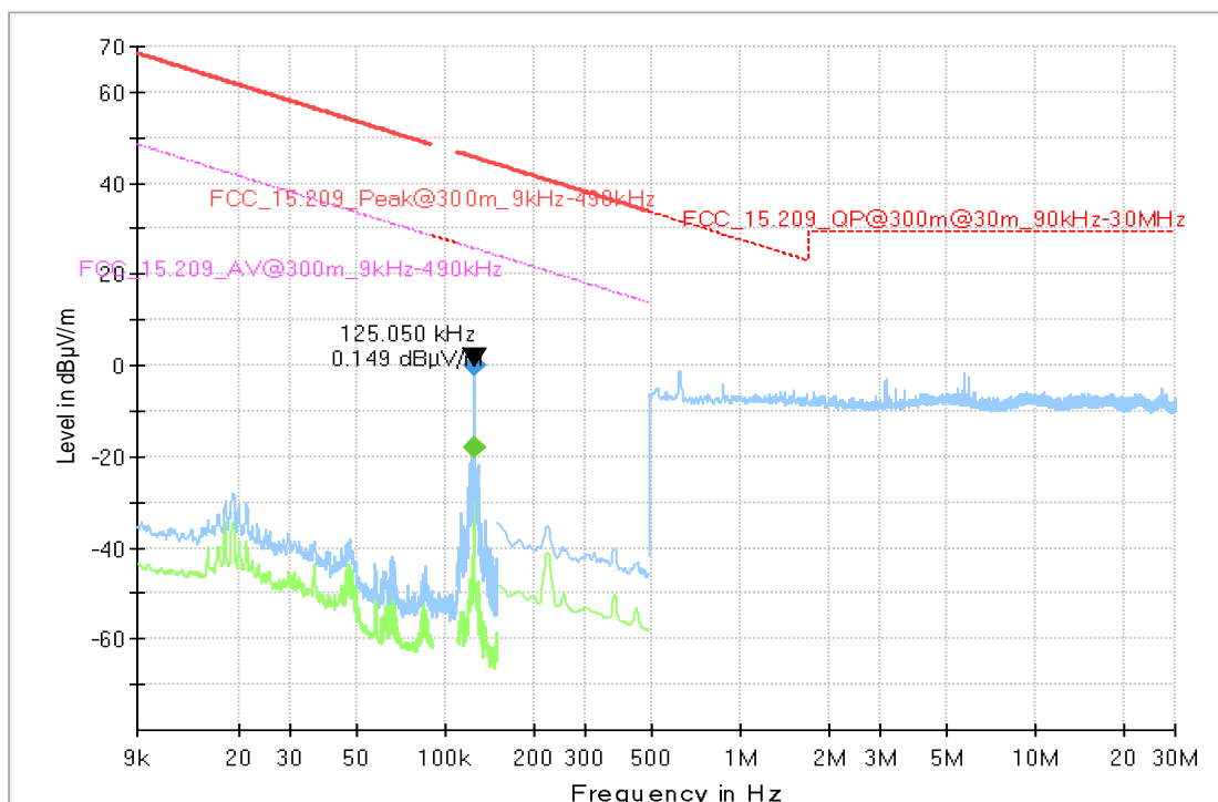
Setup_03 with immo capacitor 15 nF + Stepper motor
