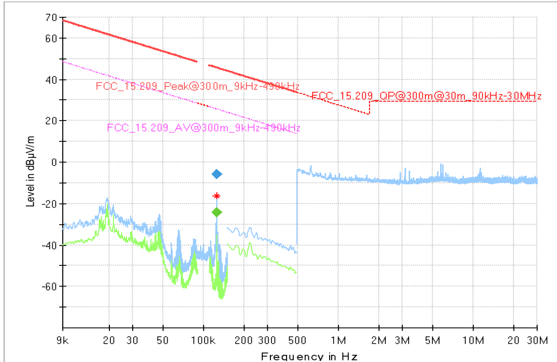
Setup_01 with immo capacitor 15 nF
