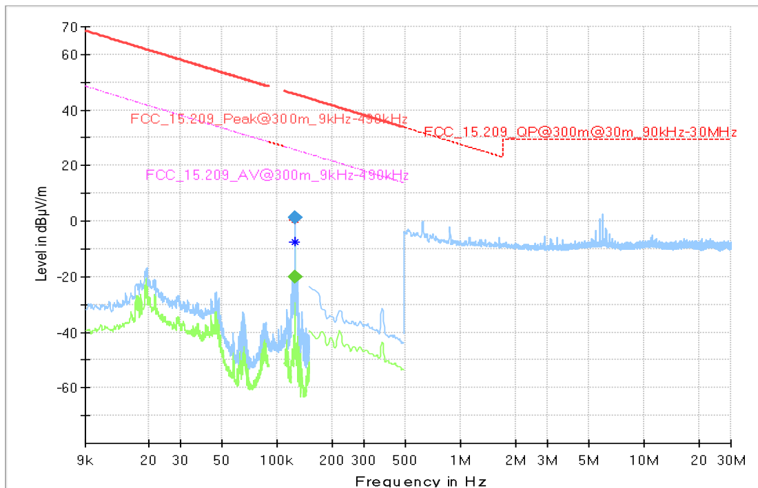
Setup_03 with immo capacitor 12 nF
