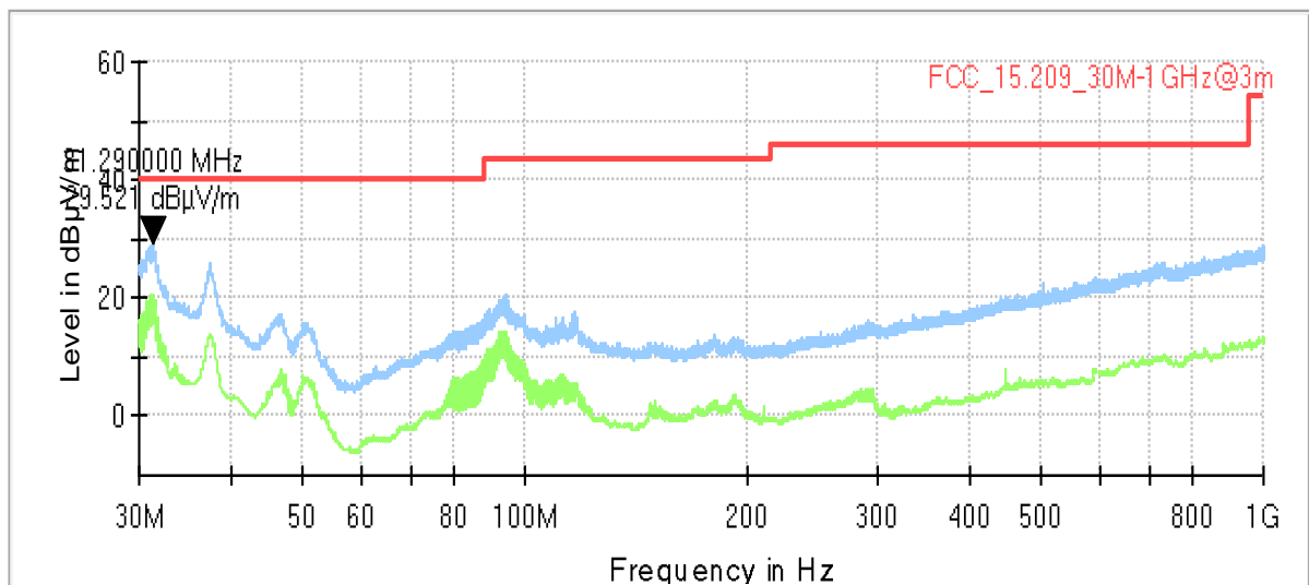
Setup_04 with immo capacitor 18 nF
