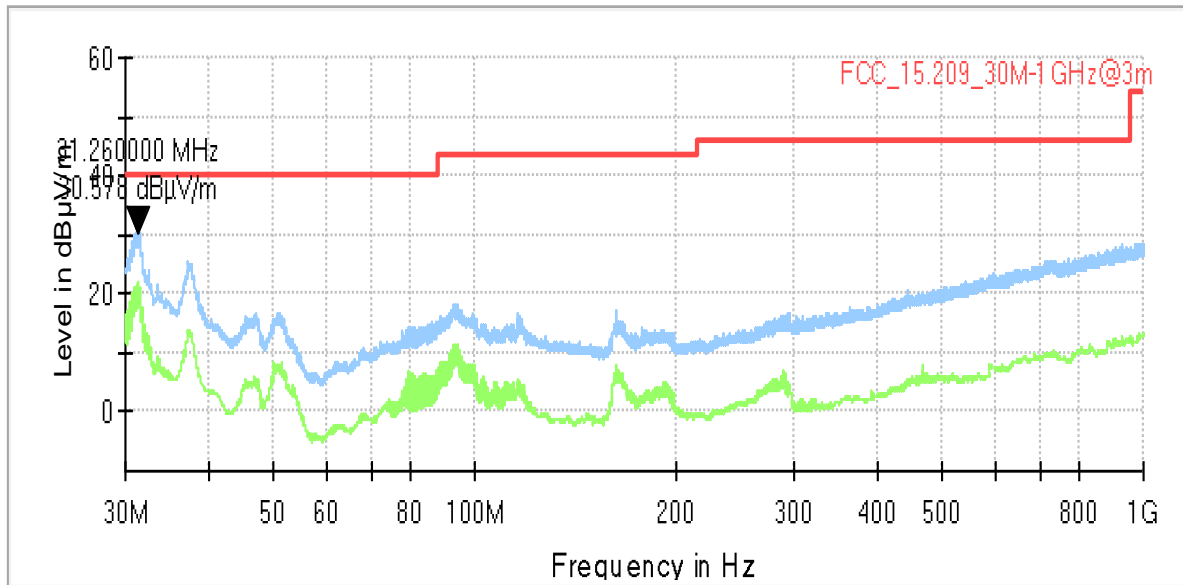
Setup_03 with immo capacitor 12 nF
