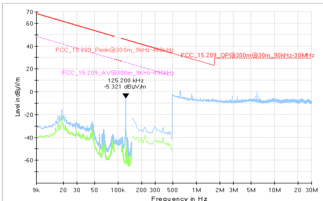
Setup_03 with Bargraph
