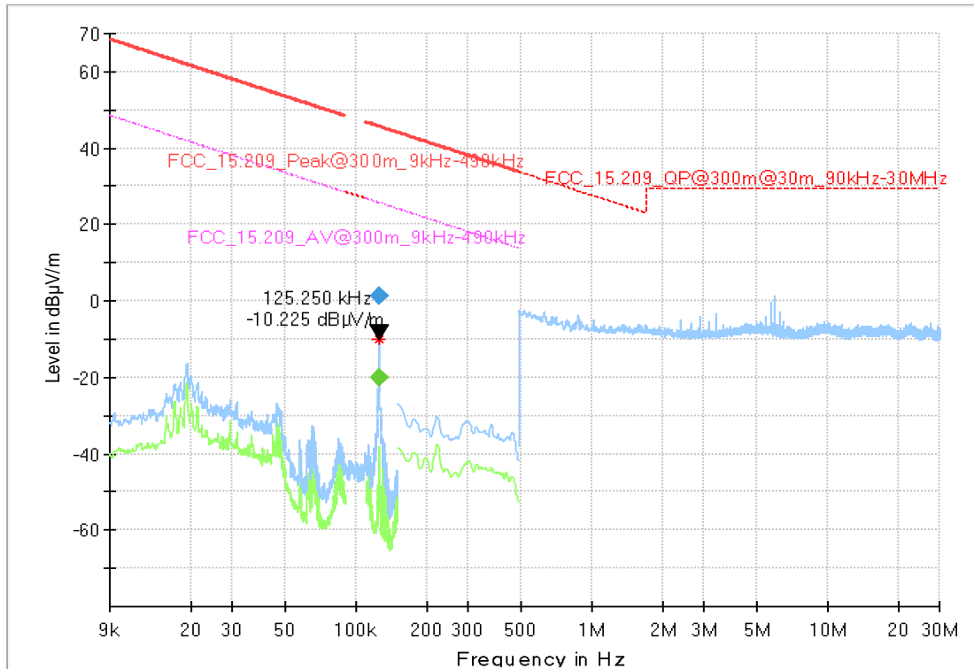
Setup_01 with Stepper motor
