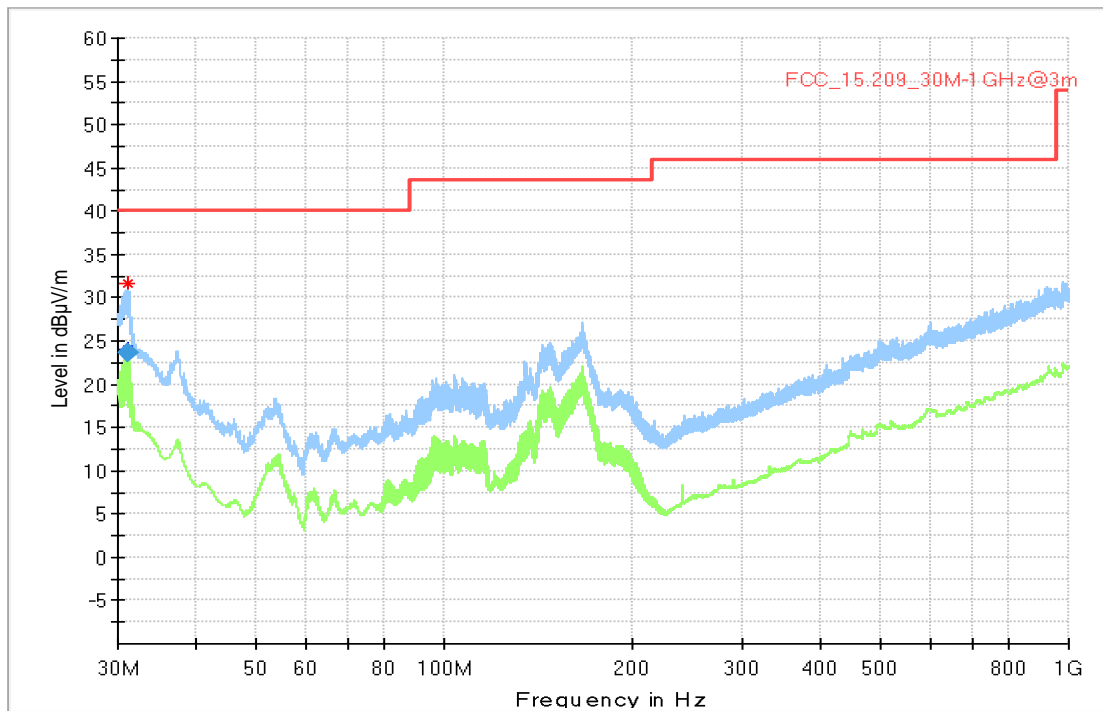
Setup_03 with Bargraph
