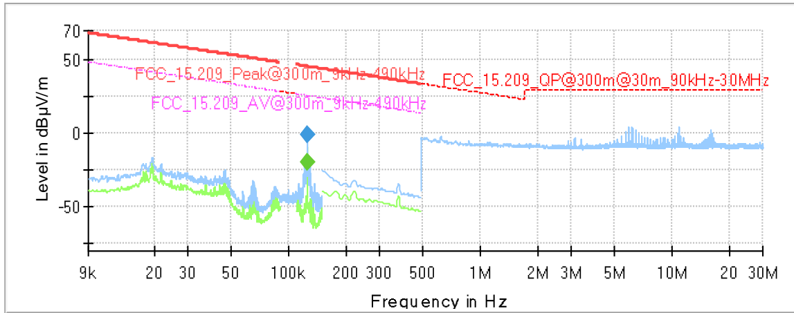
Setup_01 with immo capacitor 12nF
