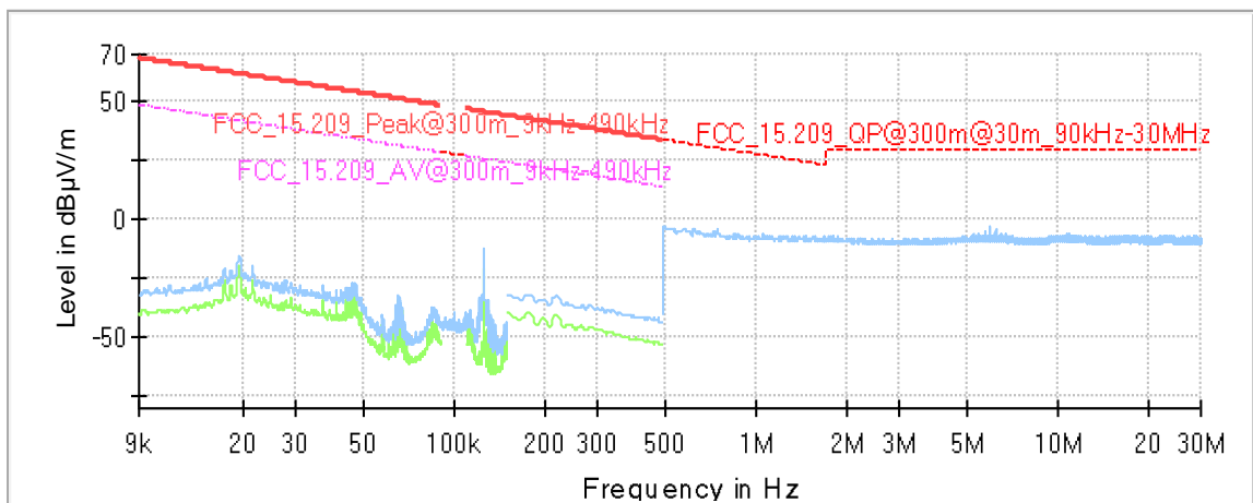
Setup_03 with immo capacitor 18nF
