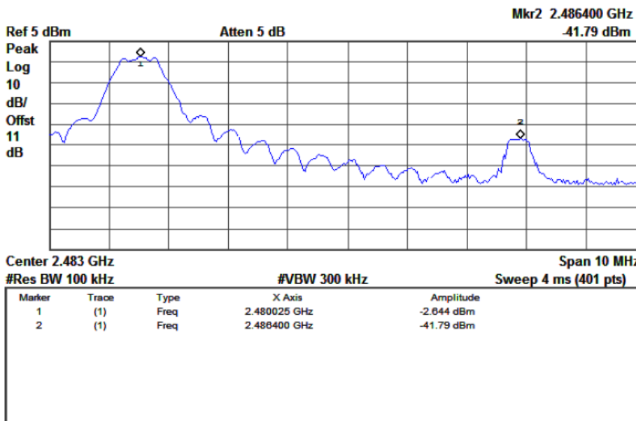
High Band Edge Plot on Channel 39
