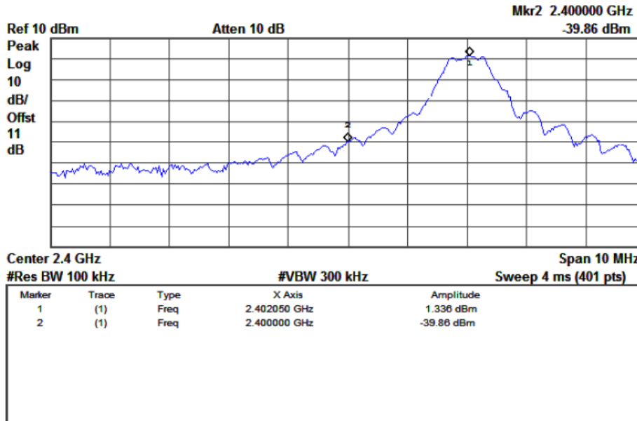
Low Band Edge Plot on Channel 00
