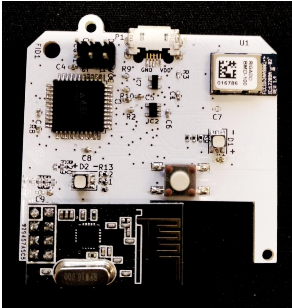
Figure 1- Dongle PCB Top
