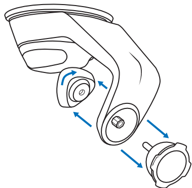
REMOVING CAR MOUNT HEAD
