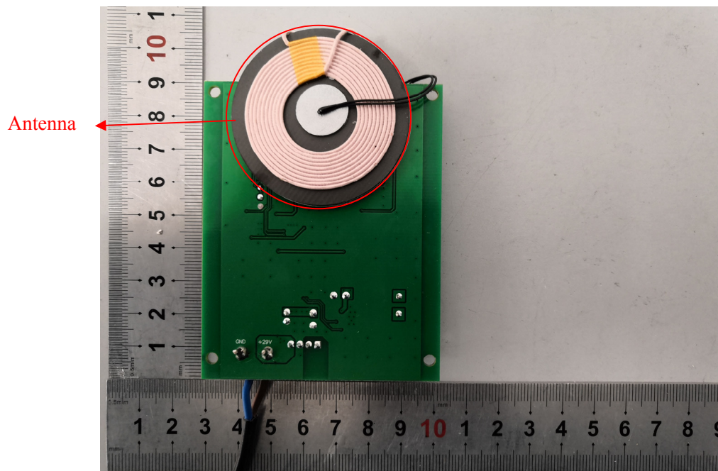
EUT – PCB-1 Bottom View
