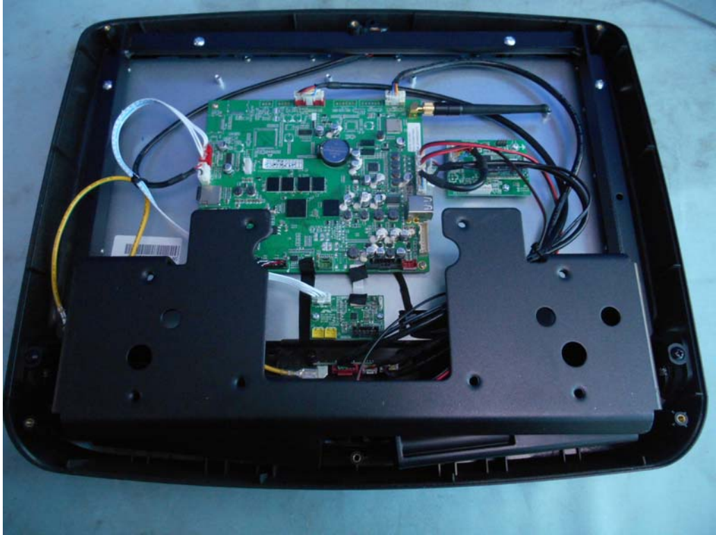
FIGURE 3 CONSOLE (M/N: XIR) COVER REMOVED
