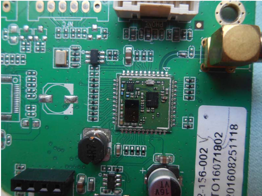
FIGURE 3 CONSOLE (M/N: XIR) CHIP & CRYSTAL ON MAIN BOARD (AP6210)
