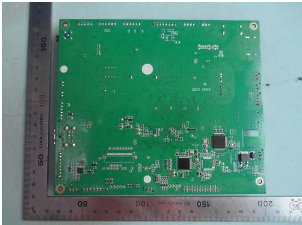
FIGURE 2 CONSOLE (M/N: XIR) MAIN BOARD (SOLDERED SIDE)
