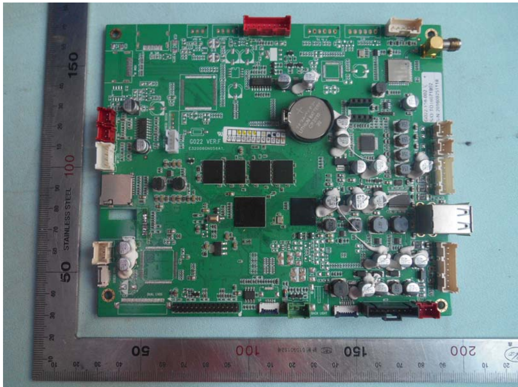
FIGURE 1 CONSOLE (M/N: XIR) MAIN BOARD (COMPONENT SIDE)
