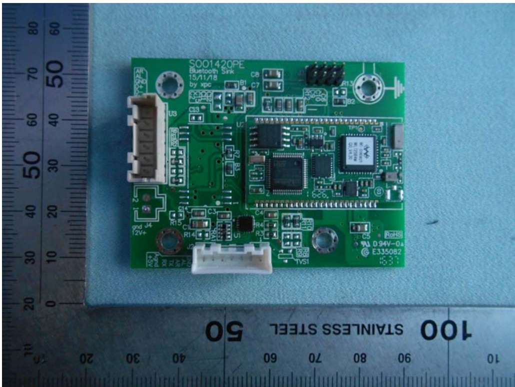
FIGURE 6 CONSOLE (M/N: XIR) MAIN BOARD #2 (COMPONENT SIDE)
