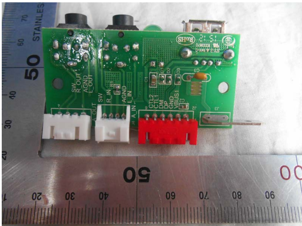
FIGURE 10 CONSOLE (M/N: XER) AUDIO BOARD (BACK VIEW)
