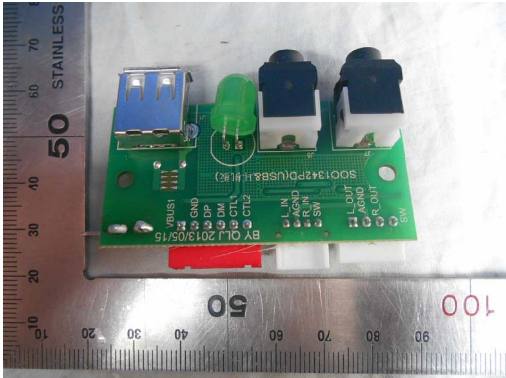
FIGURE 9 CONSOLE (M/N: XER) AUDIO BOARD (FRONT VIEW)
