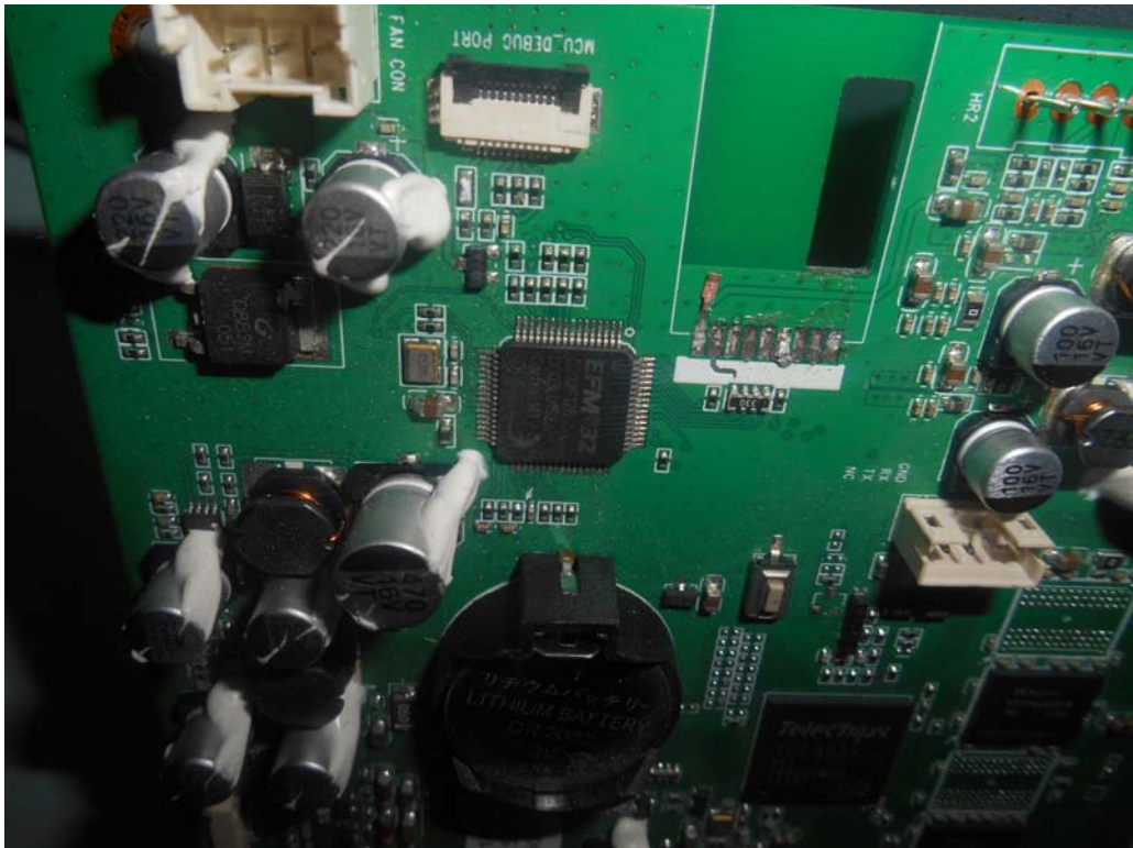
FIGURE 6 CONSOLE (M/N: XER) CHIP & CRYSTAL ON MAIN BOARD
