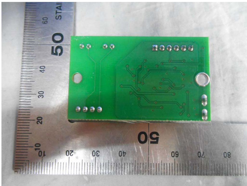
FIGURE 12 CONSOLE (M/N: XER) BOARD1 (BACK VIEW)
