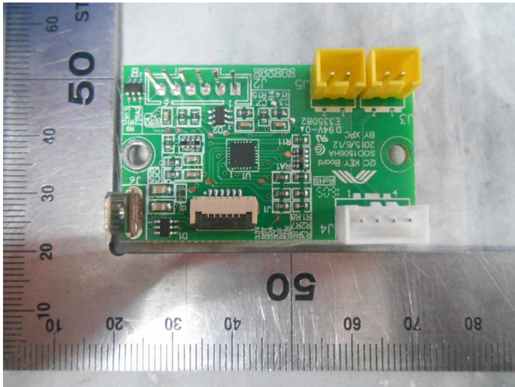
FIGURE 11 CONSOLE (M/N: XER) BOARD1 (FRONT VIEW)
