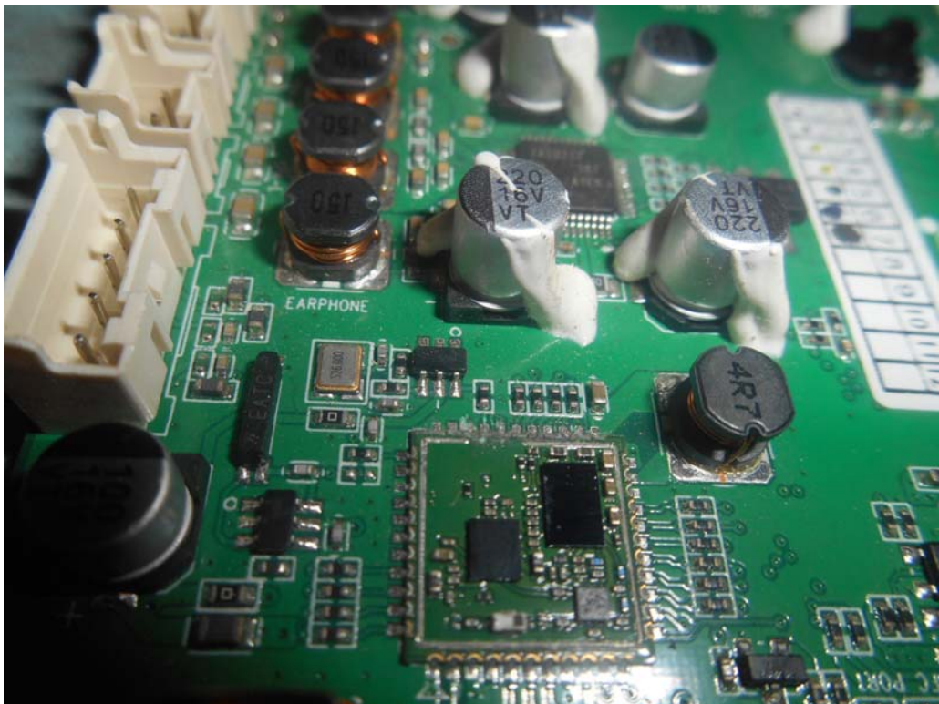
FIGURE 8 CONSOLE (M/N: XER) CHIP2 & CRYSTAL2 ON MAIN BOARD
