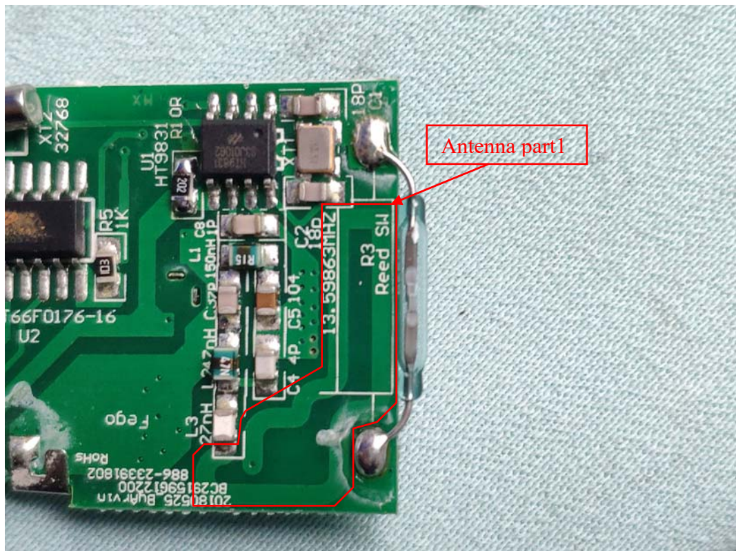
FIGURE 12 IDC CONSOLE (M/N: IDC CONSOLE) ANTENNA PART I
